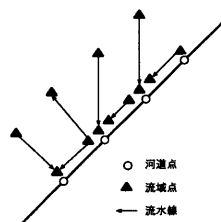
Fig. 22 Addition of new basin points
