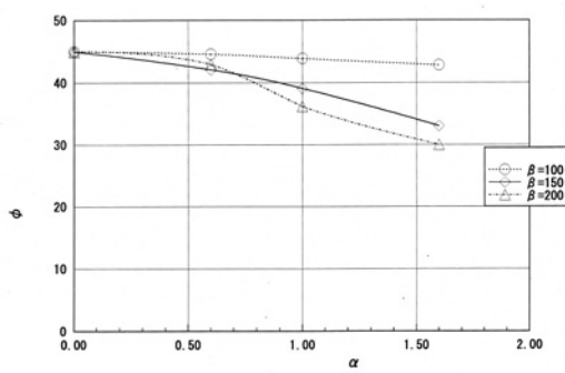
Fig.2.28 Direction of principal stress Vs. aspect ratio.
