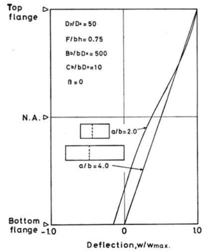
Fig.3.9 Theoretical buckling mode (transverse direction).
