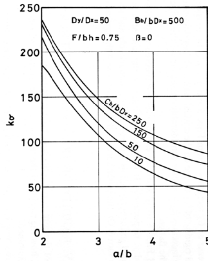
Fig.3.6 Relationship between buckling coefficient and torsional rigidity of flange.
