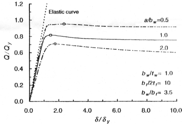
Fig.2.6 Influence of aspect ratio of web panel.
