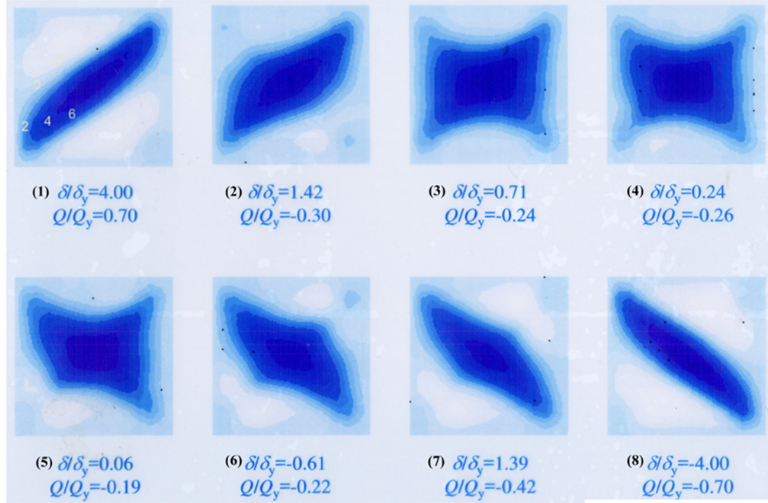
Fig.2.13 Distribution of out-of-plane deformation on web panel.
