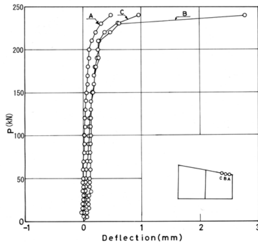
Fig.3.17 Vertical displacement of inclined flange.
