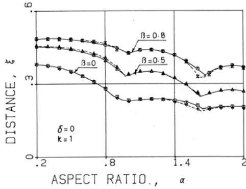
Fig. 5.8 (a) Position of equivalent bending moment.
