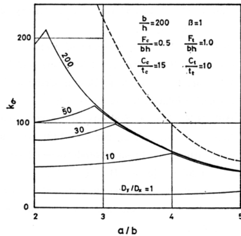
Fig.3.28 Effect of transverse stiffener.
