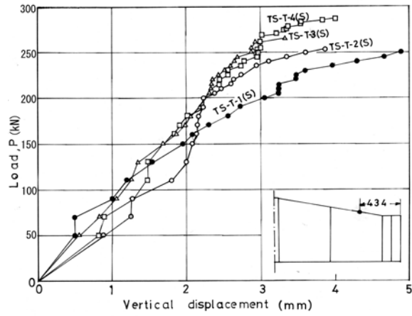
Fig.3.32 Vertical displacement of inclined flange.
