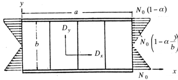
Fig.2.2 Stiffened plate.
