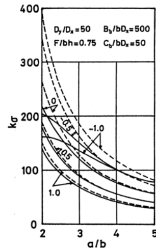
Fig.3.4 Comparison of simultaneous buckling load with value obtained by means of beam theory.
