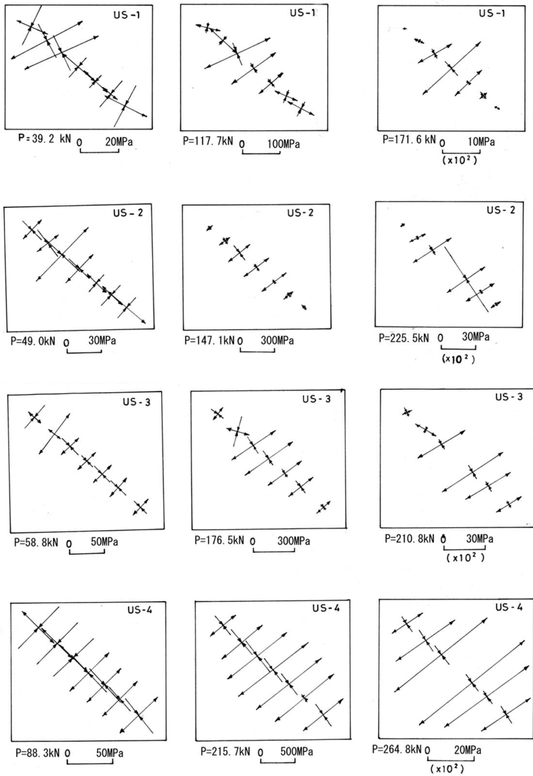
Fig.2.9 Principal stress distribution in web panel.
