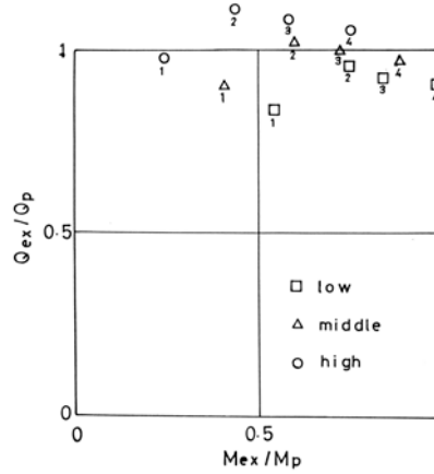
Fig.3.16 Test results.
