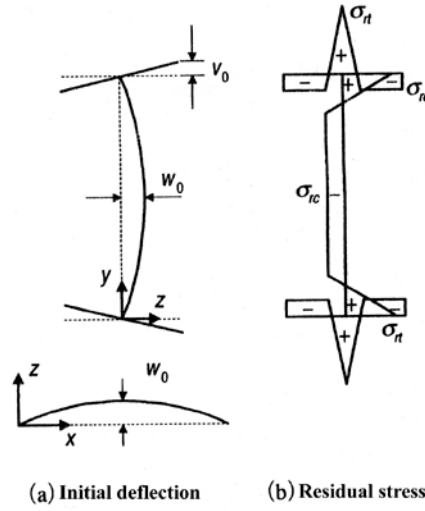
Fig.2.2 Initial imperfections.
