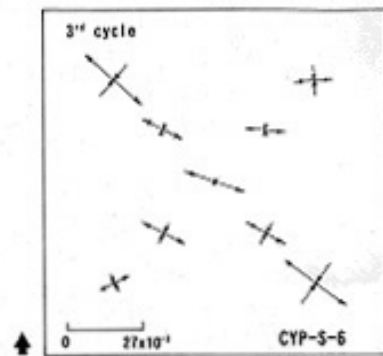
Fig.3.20. Distribution of principal strains: CYP-S-6.
