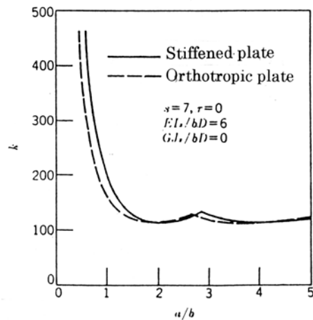
Fig.2.4 Buckling curves.
