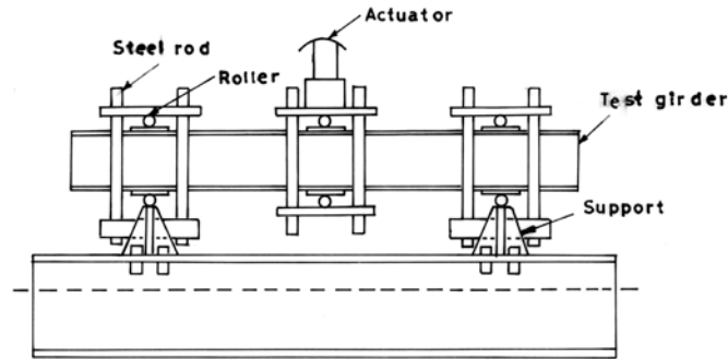
Fig.3.2 Loading apparatus.
