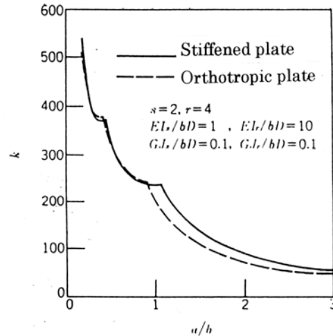
Fig.2.6 Buckling curves.
