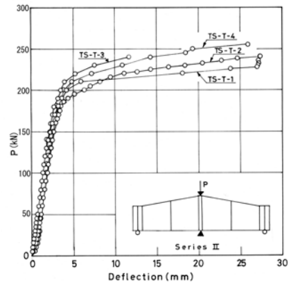
Fig.3.16 Central deflection.
