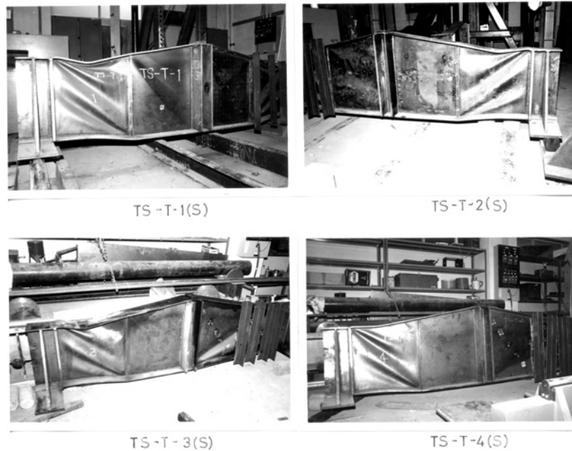
Fig.3.30 Collapsed girders.
