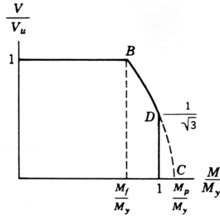
Fig.2.1 Shear-moment interaction diagrams.
