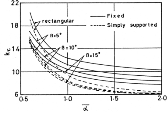
Fig.3.3 Buckling load curves.
