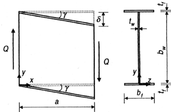
Fig.2.1 Steel girder in shear.
