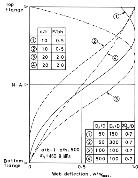
Fig.4.7 Buckling modes.
