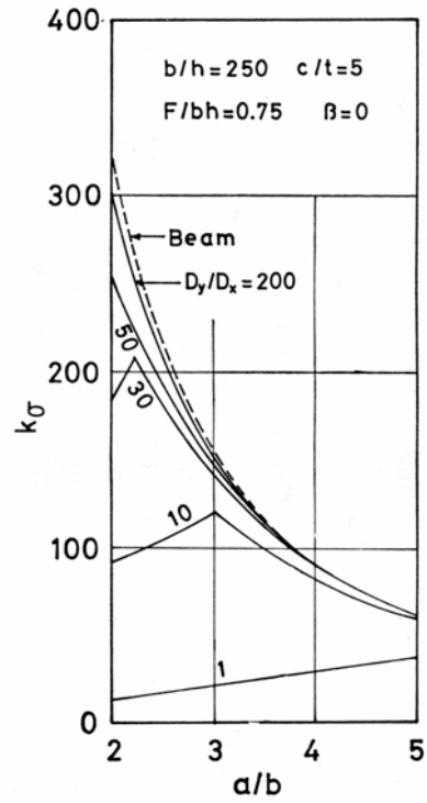
Fig.3.16 Effect of transverse stiffener.
