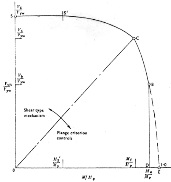
Fig.2.2 Shear-moment interaction diagrams.
