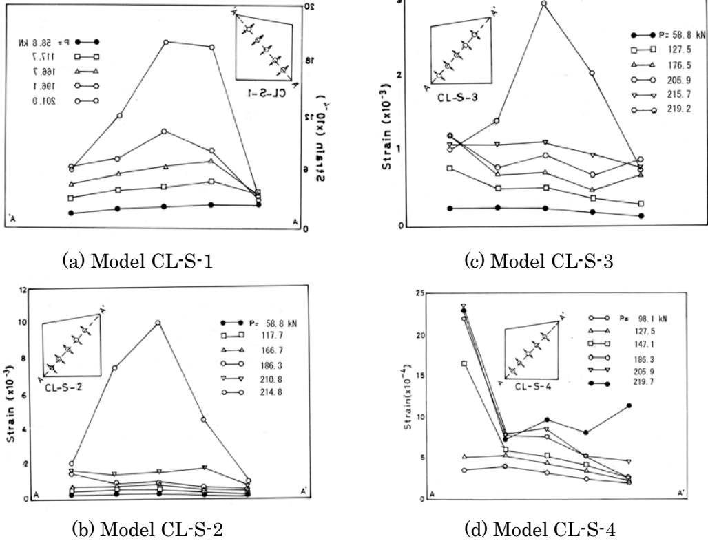
Fig.3.14 Diagonal strains on web panel.
