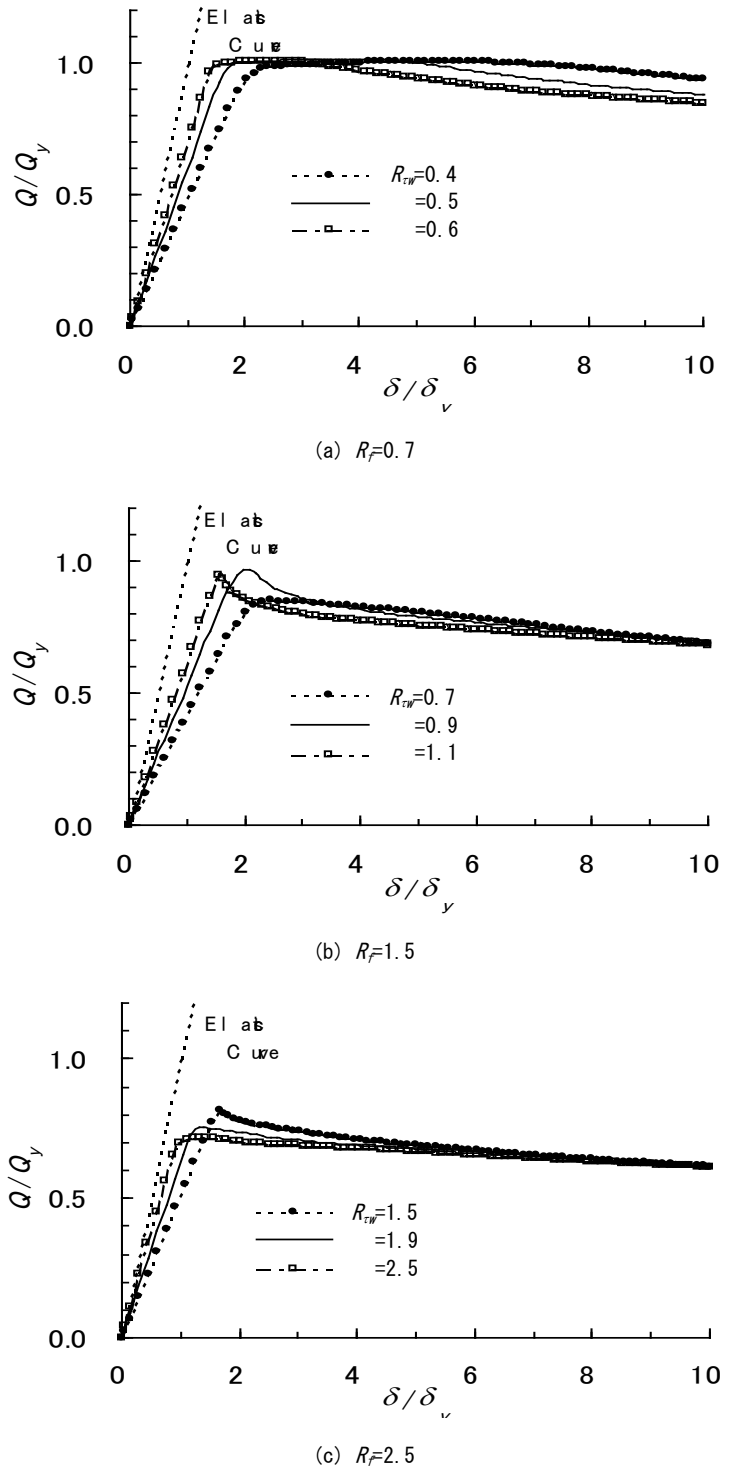
Fig.8 Shear force and displacement
