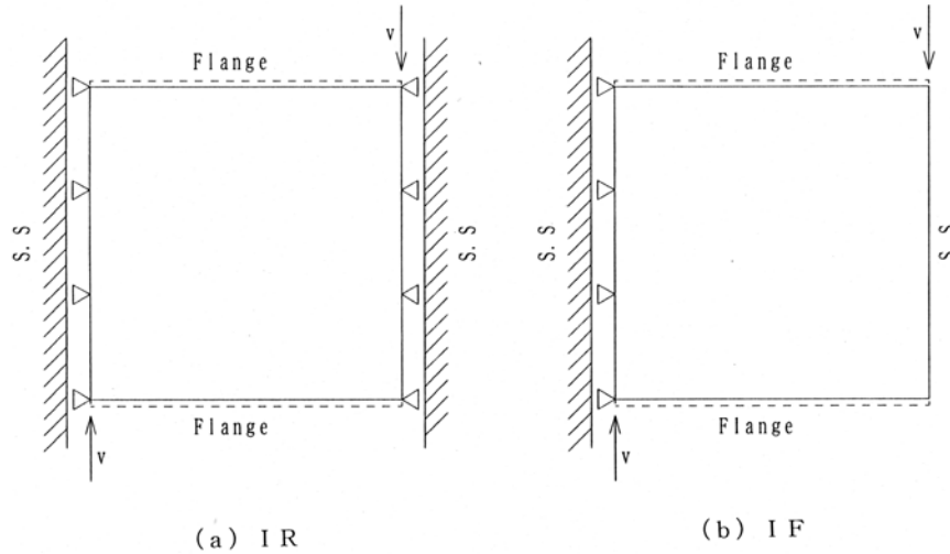
Fig.2.12 Analytical models.
