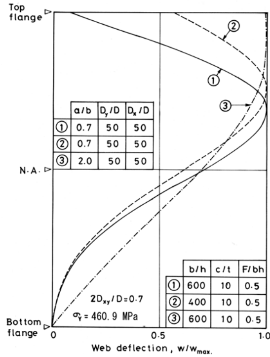
Fig.4.4 Buckling modes.
