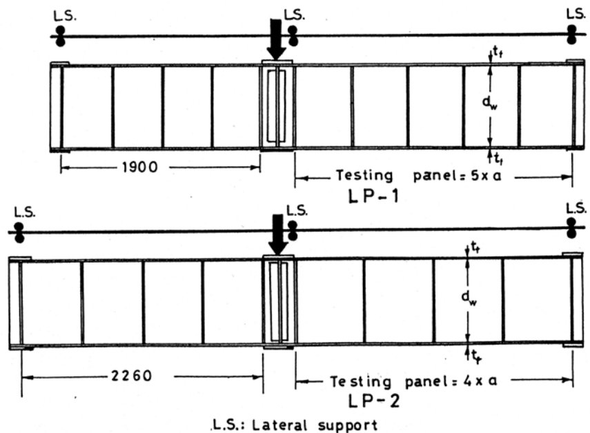
Fig.4.1 Testing plate girder models.
