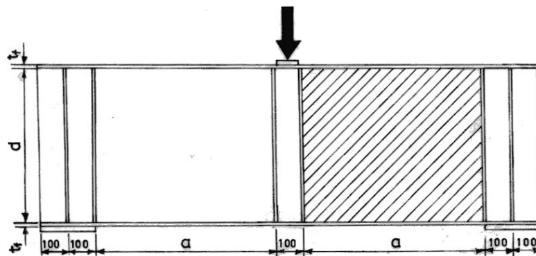
Fig. 2.1 Girder model.
