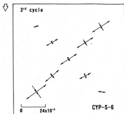
Fig.3.20. Distribution of principal strains: CYP-S-6.
