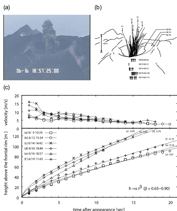
Fig. 4 (a) Snapshot of the typical rising volcanic slug. This was 10 sec after the start of the eruption at 18:57 on June 16. (b) Little change of vent position (arrows at the lower part) was observed based on the tracking of the heads of volcanic slugs during the first 10 sec of eruptions. (c) Time change of uprising velocity and height for selected 6 vigorous volcanic slugs (see figure b).
