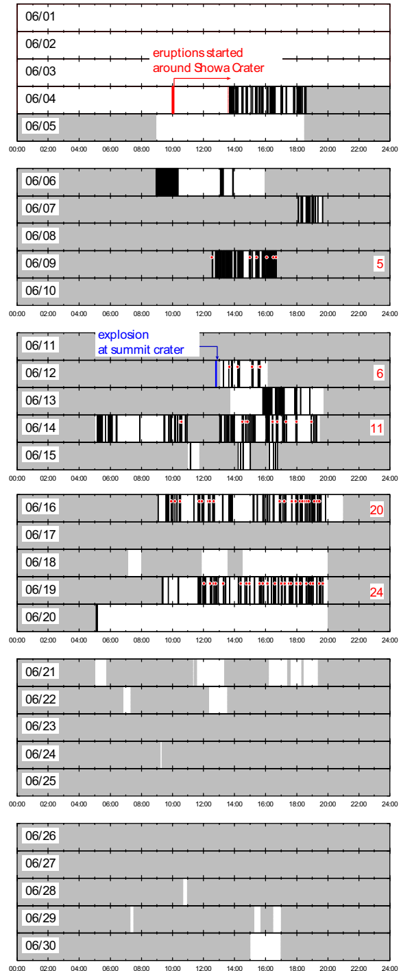
Fig. 3 Time table of the 2006 eruption determined by recorded movie images. Black and white colored areas means the occurrences of eruptions and no eruptions, respectively. Gray colored areas were the time we cannot determine whether the eruptions occurred or not due to bad weather conditions, the night time or no record of movie images. Red numbers on the day of June 9, 12, 14, 16 and 19 were the numbers of small scaled pyroclastic surges: each was occurred at the time of red circle.
