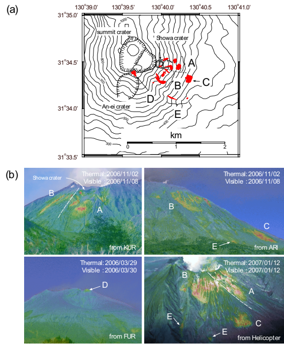
Fig. 8 (a) Five thermal anomaly areas were determined based on the results of the 2006 thermal observation. (b) Infrared thermal images overlapping on visible images taken from Kurokami branch observatory, Arimura, Furusato (see Fig. 1) and the helicopter flew over the Sakurajima volcano. Observed raw temperatures are displayed in the rainbow color scale with the constant range of 12°C.
