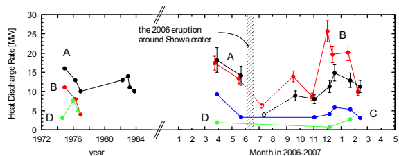
Fig. 10 Time change of estimated Q from thermal anomaly areas. Data of 1970s-1980s are from Kamo et al. (1980; 1986).
