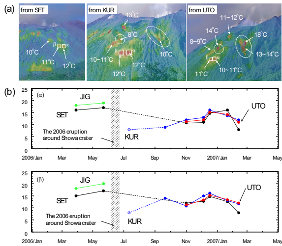
Fig. 7 (a) Infrared thermal images around Showa crater overlapping on visible images taken from three different locations. There is no large difference in the corrected difference of ground temperatures, \Delta T , except for two circled areas where we can not see same point from each location. (b) Change of \Delta T at two points, \alpha and \beta in the (a), during the 2006 observations.
