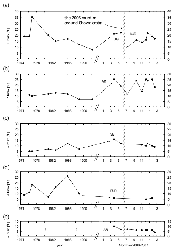
Fig. 9 Temporal change of \Delta T_{\max} at each thermal anomaly area. Data before 1990s were from Kamo and Nishi (1975) and Kamo et al. (1980; 1982; 1986; 1988; 1989; 1995).
