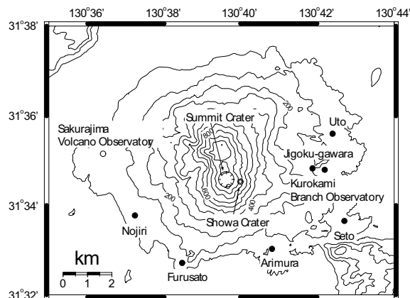
Fig. 1 Map of Sakurajima volcano with the locations of 2006 infrared thermal observations. The 2006 eruptions around Showa crater was observed from Jigoku-gawara and Kurokami branch observatory with the video cameras.
