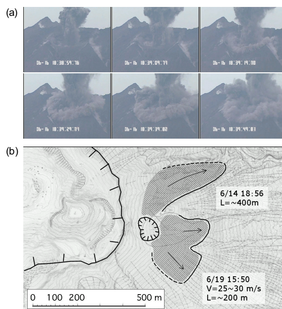
Fig. 5 (a) Snapshots with 10 sec intervals of typical small scaled pyroclastic surges occurred at the 2006 eruptions. Almost all surges were made by the collapse of volcanic cloud. (b) Two largest surges run out 200~400 m from the crater rim.
