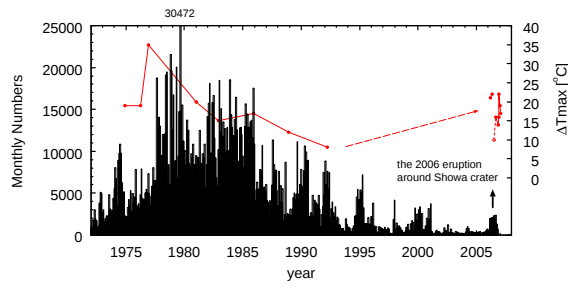
Fig. 2 Monthly Number of B-type earthquakes occurred at Sakurajima volcano from 1972 to 2006. Red line with points is \Delta T_{\max} at the thermal anomaly area around Showa crater.
