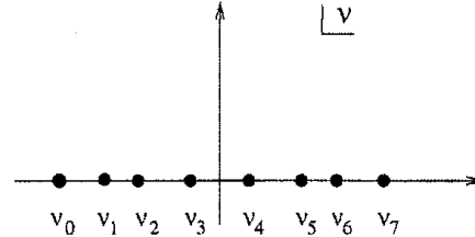
Figure 2: The \nu_i 's are real for the ground state.
