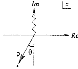
Figure 3: The branch cut, and a ray in the complex x -plane.
