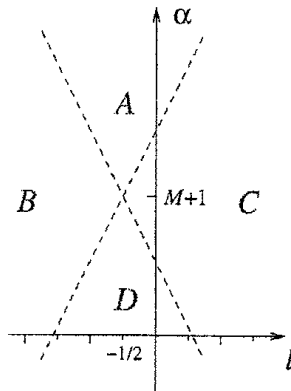
Figure 8: The ‘phase diagram’ at fixed M .
