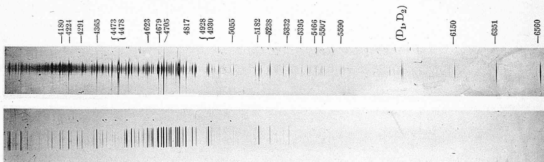
Fig. 3 (Blue discharge)
