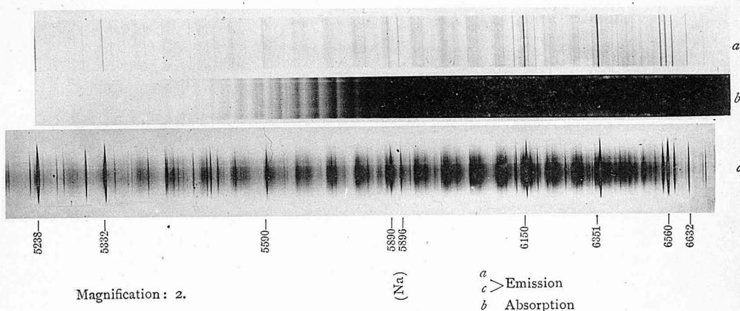
Fig. 5 (Bromine Band Spectrum)
