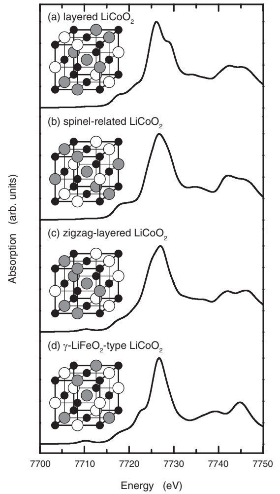
FIG. 5. Calculated Co-K XANES of ordered rocksalt LiCoO 2 polymorphs of (a) O3-type layered rocksalt, (b) spinel-related type, (c) zigzag-layered type, and (d) \gamma -LiFeO 2 type. Schematic images of the corresponding Li/Co arrangements are also shown. Open, gray, and small black spheres denote Li, Co, and O ions, respectively.
