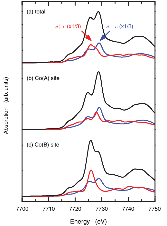
FIG. 3. (Color online) Calculated Co- K XANES of (a) total, (b) Co(A) site, and (c) Co(B) site of O4-LiCoO 2 with their orientation dependence.
