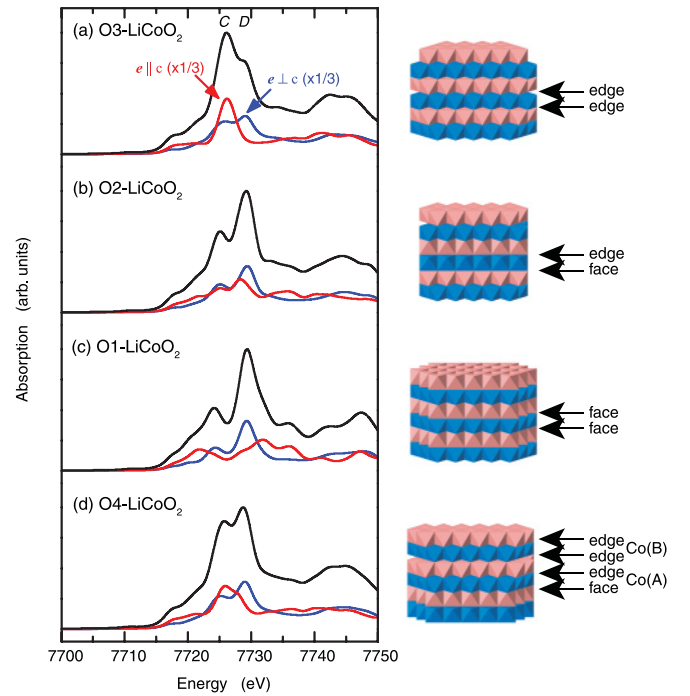
FIG. 2. (Color online) Calculated Co-K XANES of layered LiCoO 2 with the stacking sequence of (a) O3, (b) O2, (c) O1, and (d) O4 types with their orientation dependence. Schematic images of the corresponding stacking sequences are also shown. Blue and red polyhedra denote CoO 6 and LiO 6 octahedra, respectively.
