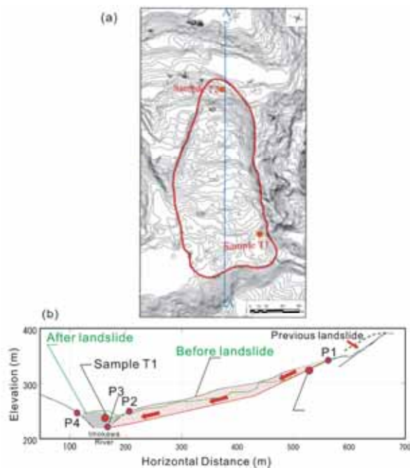
Fig. 9 Plan and Section of the Terano landslide (a: Plan obtained from air bone lazax scanner. Contour lines are 2m pitch. b: Central section A-A of the Fig.9a)
