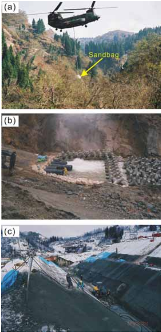
Fig. 17 Emergency measures to prevent failure of the Higashi Takezawa landslide dam. (a) Helicopters of the Japanese Self-Defense Force carried sandbags and piled them on the lowest part of the landslide dam crest every several minutes during our observation, (b) and (c) Diversion pipe lines and open-channel spillway constructed by the Ministry of Land, Infrastructure and Transportation
