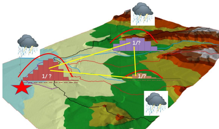
Figure 1 Spatial temporal correlation problem for flood risk assessment
