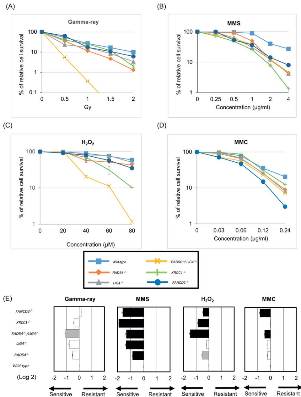
Fig. 2. Sensitivity of DNA-repair-deficient TK6 mutant cells to \gamma -rays (A), MMS (B), H 2 O 2 (C), and MMC (D) as measured via colony formation assay. The error bars represent SD from three independent experiments. (E) Sensitivity profiles of the indicated DNA-damaging agents in the selected DNA repair-deficient TK6 panel. Negative (the left side) and positive (the right side) scores indicate that the indicated cells are
