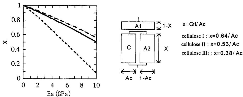
Fig. 1. Relationship of X and amorphous Young's modulus. cellulose I : ———; cellulose II : ————; cellulose III I : - - - -; A1, A2 : amorphous component; C : crystalline component.
