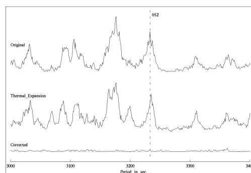
Fig.6 Spectra in the period range from 3000 to 3400 seconds. The layout of the figure is same as Fig.4.
