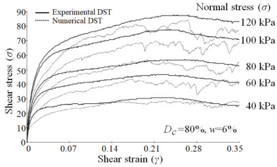
Fig. 10 Shear stress – shear strain curves under different normal pressures for the humid sand
