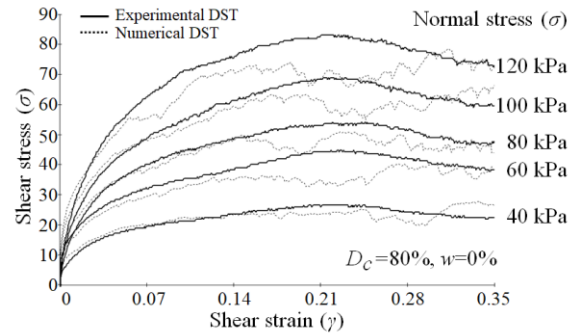
Fig. 9 Shear stress – shear strain curves under different normal pressures for the dry sand
