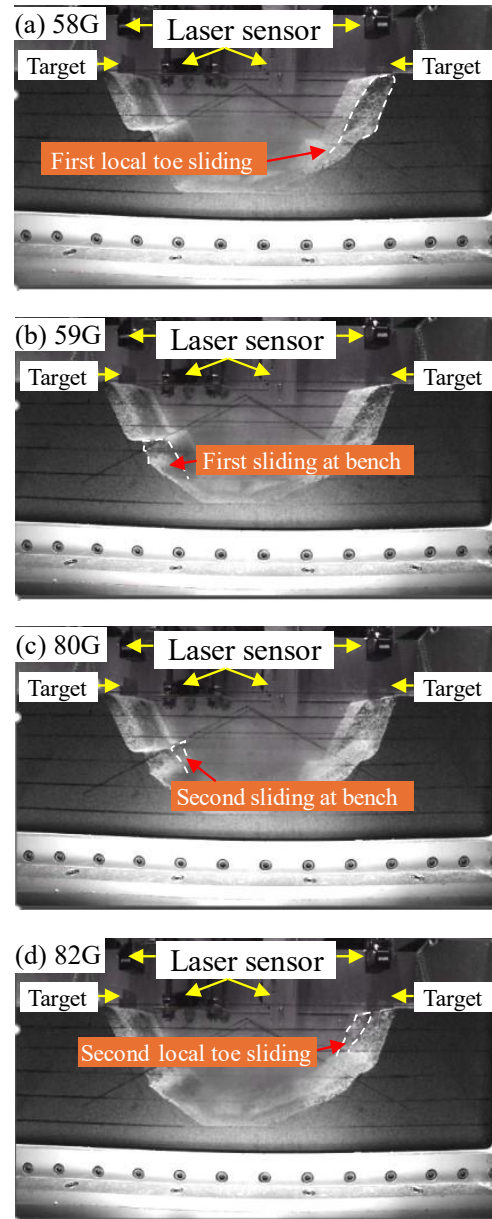
Fig. 5 Process of sliding of benched slopes with increasing centrifugal acceleration
