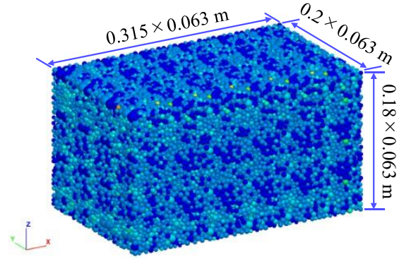
Fig. 11 Dimensions of the foundation in DEM
