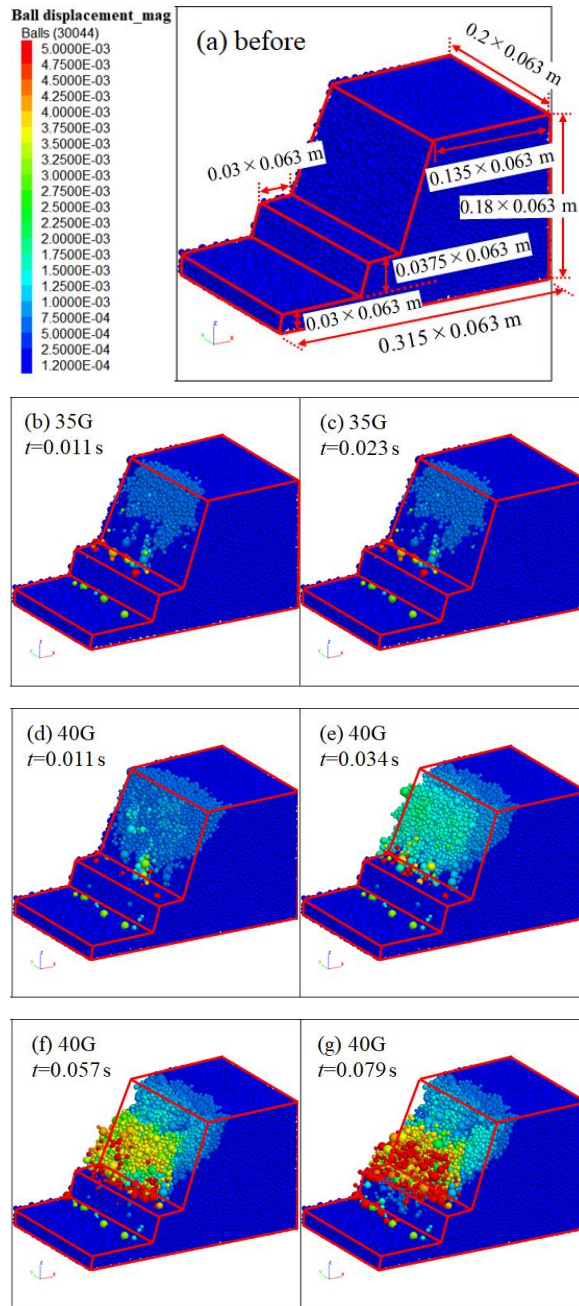
Fig. 12 Sliding process of benched slopes with the lower bench simulated by DEM
