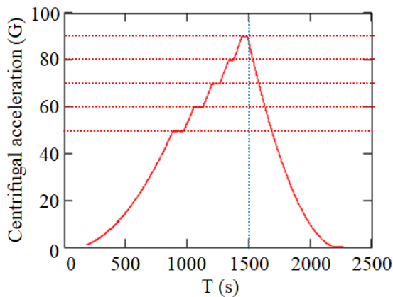
Fig. 4 Centrifugal acceleration with respect to time
