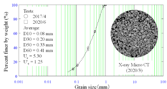
Fig. 2 Grain size distribution of Hiroshima sand after removal of grain size larger than 1 mm
