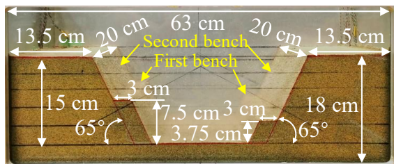
Fig. 1 Physical model used in the centrifuge test (model scale)
