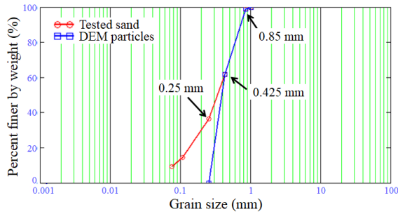
Fig. 8 Comparison of grain size distribution curves between real sand and DEM particles
