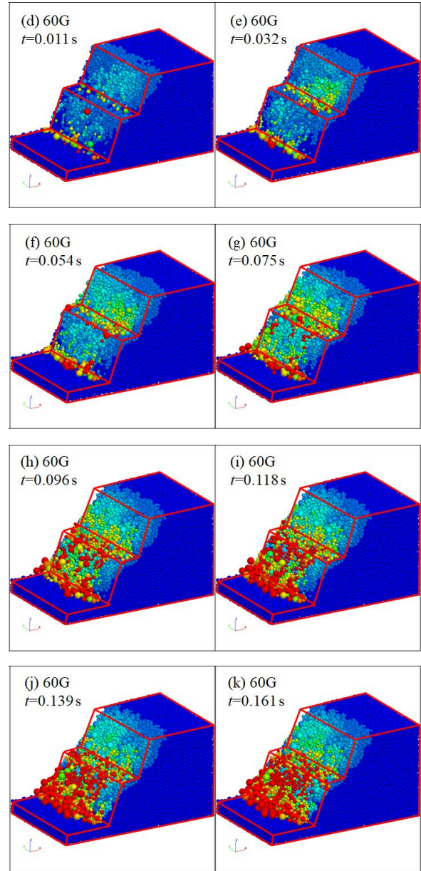
Fig. 13 Sliding process of benched slopes with the higher bench simulated by DEM
