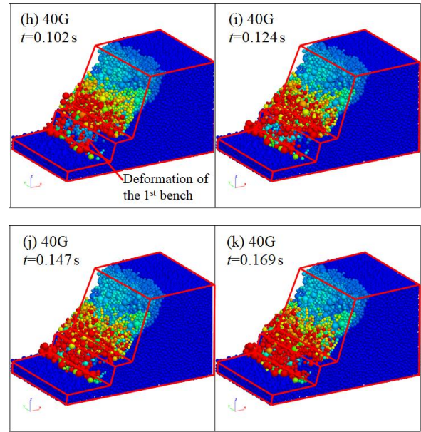
Fig. 12 Sliding process of benched slopes with the lower bench simulated by DEM
