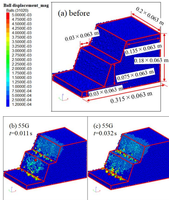
Fig. 13 Sliding process of benched slopes with the higher bench simulated by DEM
