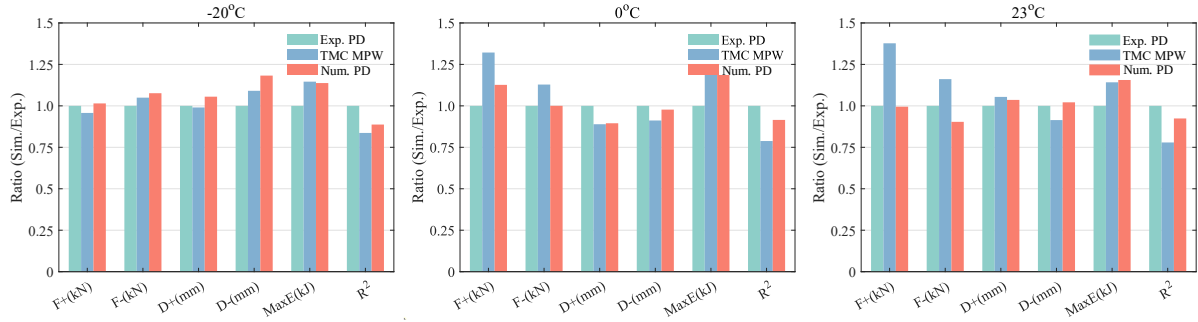
Figure 5.14 Validation of pseudo-dynamic hybrid simulation: F^{+}(-) : maximum (minimum) force; D^{+}(-) : maximum (minimum) displacement; \text{MaxE} : energy dissipation of maximum loop; R^2 : coefficient of determination.
