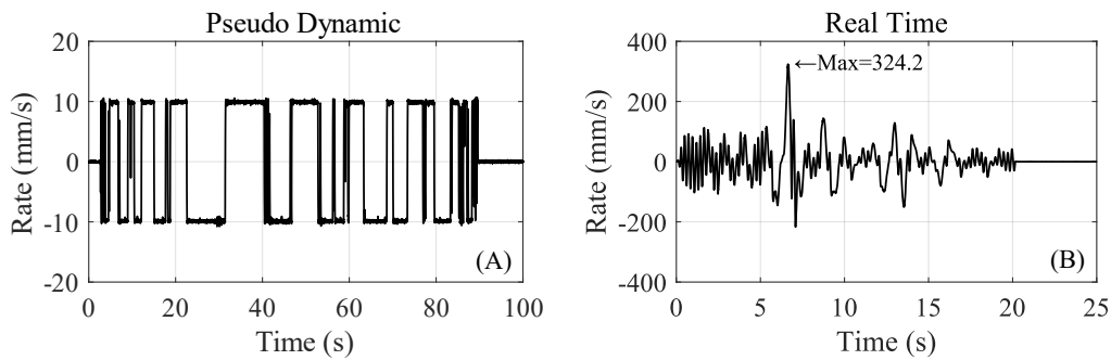
Figure 3.15 Rate of (A) pseudo-dynamic and (B) real-time hybrid simulations.
