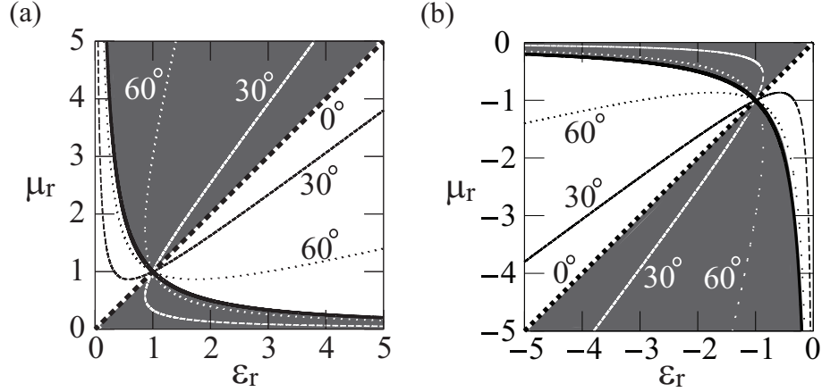
Figure 3.2: Brewster's condition for media with relative permittivity \varepsilon_r and relative permeability \mu_r . Brewster's condition exists in the (a) first and (b) third quadrants of the (\varepsilon_r, \mu_r) -plane. Brewster's conditions for TE and TM waves exist in the shaded and unshaded areas, respectively. All the lines except the bold solid line represent the contour lines of the Brewster angles. The bold solid line and the bold dashed line correspond to \varepsilon_r \mu_r = \pm 1 and \varepsilon_r = \mu_r , namely, n = \pm 1 and Z_r = 1 , respectively.
