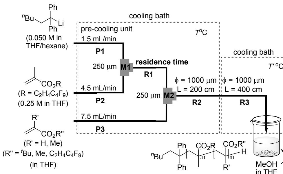
Scheme 2. Flow microreactor system for anionic polymerization of perfluoroalkyl methacrylates initiated by 1,1-diphenylhexyllithium. T-shaped micromixer: M1 and M2 ; Microtube reactor: R1 , R2 and R3 .
