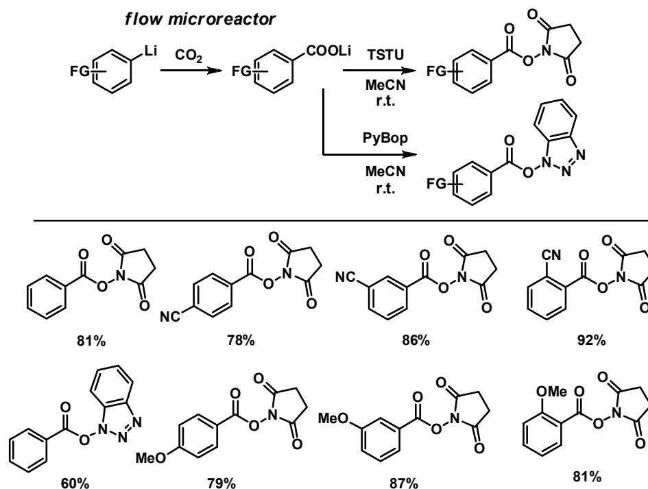
Figure 1. Flow microreactor synthesis of active esters.
