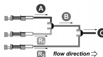
Figure 2. Classification of integrated synthesis. A: Starting material, B: intermediate, C: product, R 1 and R 2 : reagents.
