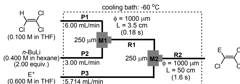
Scheme 3. A flow microreactor system for the H/Li exchange of trichloroethene with n -BuLi (2.00 eq) and the subsequent reaction with electrophiles. T-shaped micromixers: M1 and M2 , microtube reactors: R1 and R2 .
