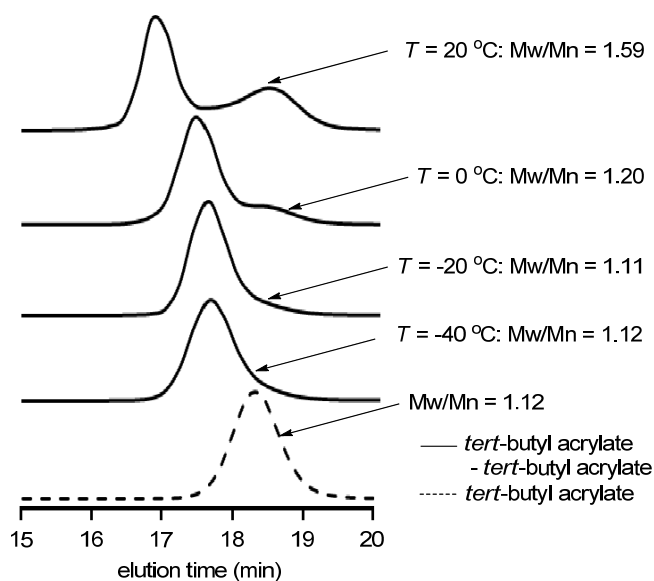
Figure 2. Size exclusion chromatography traces of sequential anionic polymerization of tert -butyl acrylate in the integrated flow microreactor system. Effect of reaction temperature ( T ) in t^{R2}=2.24 s.
