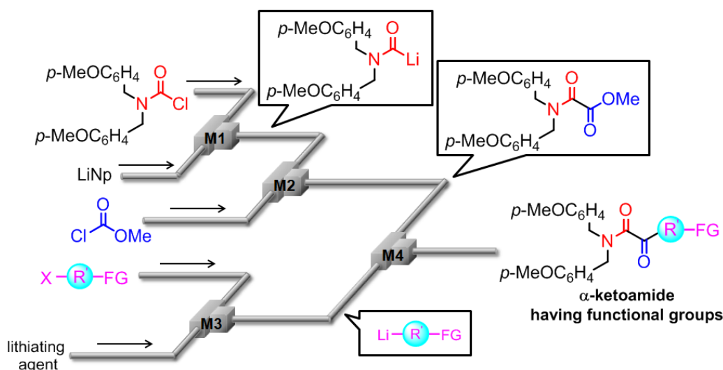
Figure 3. Three-component synthesis using carbamoyllithium, methyl chloroformate and unstable organolithiums.
