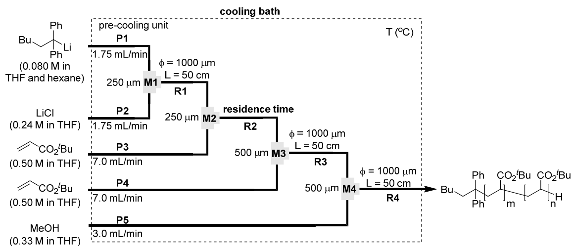
Scheme 2. A flow microreactor system for the Sequential anionic polymerization of tert -butyl acrylate initiated by 1,1-diphenylhexyllithium. T-shaped micromixer: M1 , M2 , M3 and M4 . Microtube reactor: R1 , R2 , R3 and R4 .
