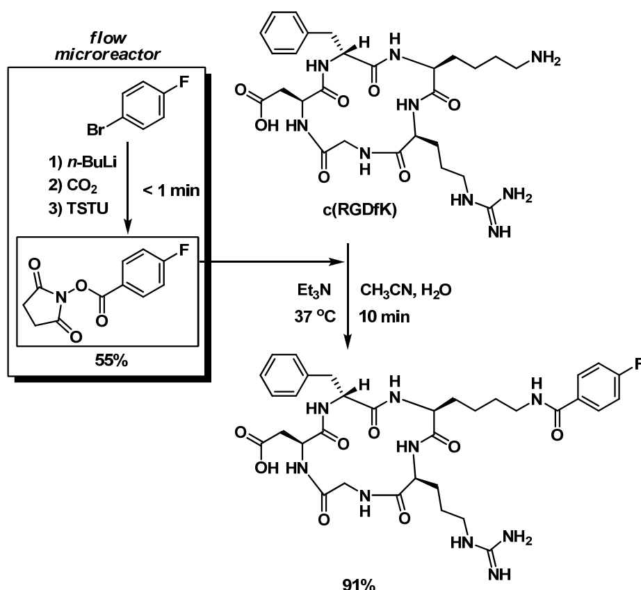
Figure 2. Coupling reaction of cyclo (Arg-Gly-Asp-D-Phe-Lys) (c(RGDfK)) with N -succinimidyl-4-fluorobenzoate (SFB).
