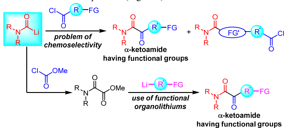
Figure 2. Synthesis of \alpha -ketoamides having functional groups via carbamoyllithiums
