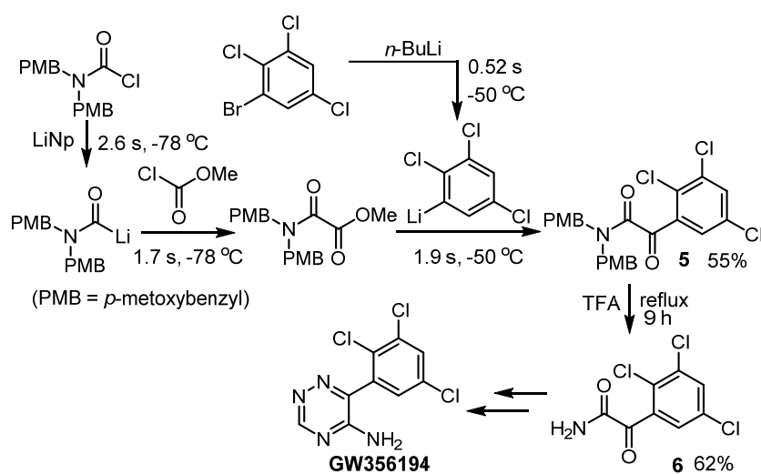
Figure 4. Formal synthesis of GW356194.
