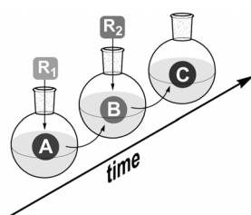
Figure 2. Classification of integrated synthesis. A: Starting material, B: intermediate, C: product, R 1 and R 2 : reagents.
