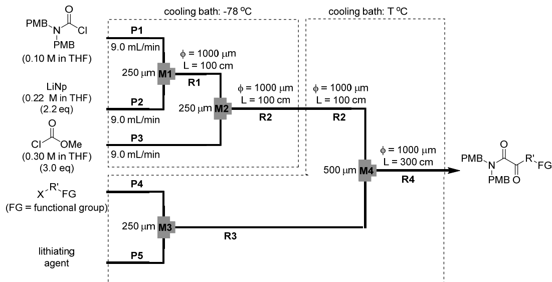
Figure 3. An integrated flow microreactor system for the three-component coupling of carbamoyllithiums, methyl chloroformate, and functional organolithiums. T-shaped micromixers: M1 , M2 , M3 , and M4 , microtube reactors: R1 , R2 , R3 , and R4 .
