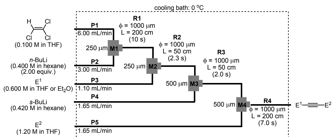
Scheme 2. An integrated flow microreactor system for the synthesis of unsymmetrically disubstituted ethynes by sequential introduction of two electrophiles. T-shaped micromixers: M1 , M2 , M3 , and M4 , microtube reactors: R1 , R2 , R3 , and R4 .
