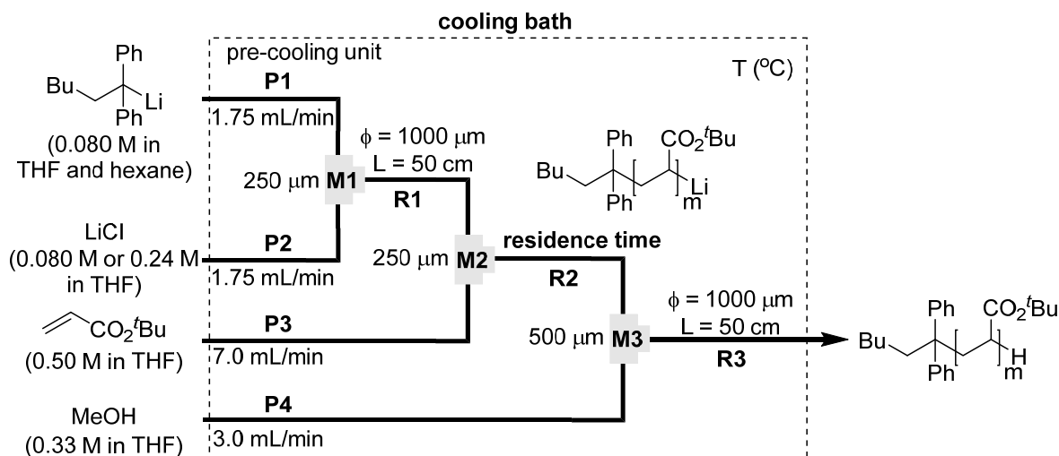
Scheme 1. A flow microreactor system for anionic polymerization of tert -butyl acrylate initiated by 1,1-diphenylhexyllithium. T-shaped micromixer: M1 , M2 and M3 . Microtube reactor: R1 , R2 and R3 .
