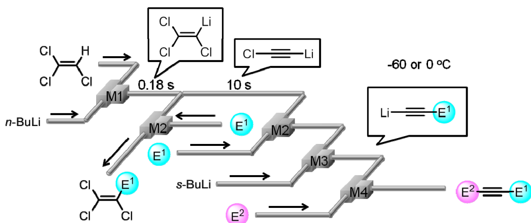
Figure 4. Selective synthesis of alkenes and alkynes by switching of the reaction-pathways of trichlorovinyl lithium based on the residence time control.
