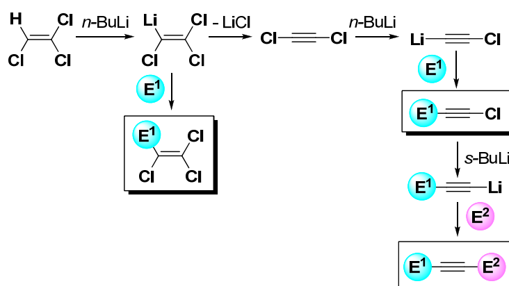
Figure 1. Synthesis of chloroalkenes and alkynes from trichloroethene.
