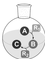
Figure 2. Classification of integrated synthesis. A: Starting material, B: intermediate, C: product, R 1 and R 2 : reagents.
