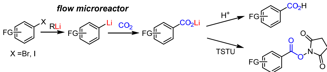
Figure 5. Synthesis of carboxylic acids and active esters by carboxylation of functional aryllithiums using \text{CO}_2 gas.
