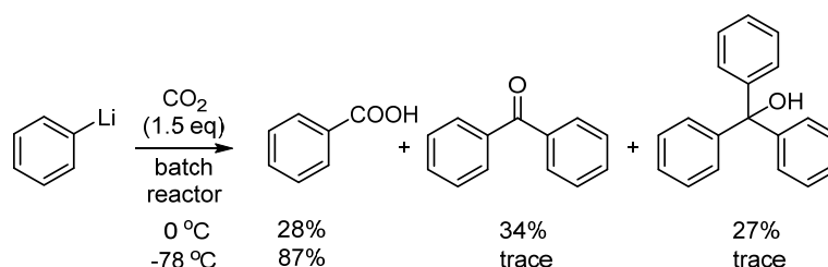
Scheme 2. Reaction of phenyllithium with carbon dioxide using a conventional macro batch reactor.
