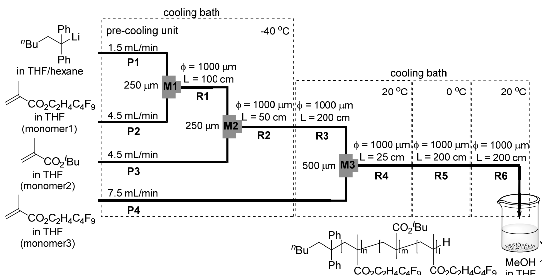
Scheme 3. Integrated flow microreactor system Triblock anionic polymerization of 2-(nonafluorobutyl)ethyl methacrylate (NFBEMA), tert -butyl methacrylate (tBuMA), and 2-(nonafluorobutyl) ethyl methacrylate (NFBEMA) initiated by 1,1-diphenylhexyllithium. T-shaped micromixer: M1 , M2 and M3 ; Microtube reactor: R1 , R2 , R3 , R4 , R5 and R6 .
