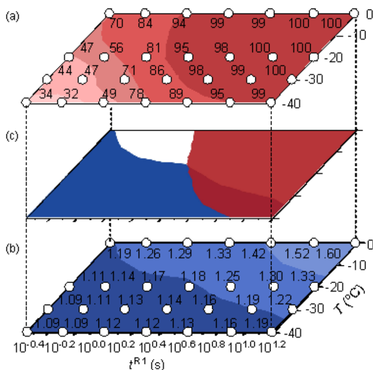
Figure 2. Temperature–residence time (in R1 ) map for the sequential anionic polymerization of 2-(nonafluorobutyl)ethyl methacrylate initiated by 1,1-diphenylhexyllithium in flow microreactors. (a) Contour map with scatter overlay of the conversion of 2-(nonafluorobutyl)ethylmethacrylate in the first polymerization of 2-(nonafluorobutyl)ethylmethacrylate, which is indicated by numbered circles; (b) contour map with scatter overlay of the Mw/Mn in the sequential polymerization of 2-(nonafluorobutyl)ethyl methacrylate, which is indicated by numbered circles; and (c) the domain that gave high conversion (>95 %) and narrow Mw/Mn ( Mw/Mn < 1.2 )
