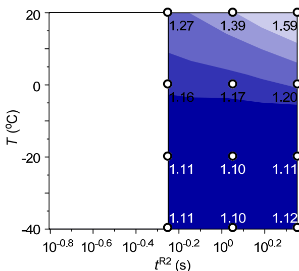
Figure 3. Temperature-residence time map for the sequential anionic polymerization reactions of tert -butyl acrylate initiated by 1,1-diphenylhexyllithium in a flow microreactor system. Contour plots with scatter overlay of the molecular-weight distribution, which are indicated by numbered circles.
