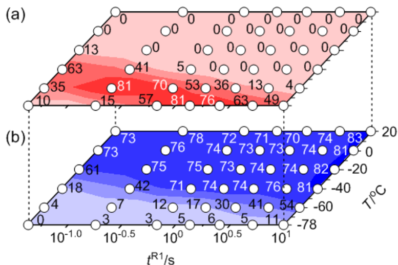
Figure 2. Effects of temperature ( T ) and residence time ( t^{R1} ) for H/Li exchange of trichloroethene with n -BuLi (2.00 eq) followed by the reaction with benzaldehyde using the flow microreactor system. (a) Contour map with scattered overlay of the yield of 2,3,3-trichloro-1-phenylprop-2-en-1-ol ( 1 ), and (b) contour map with scattered overlay of the yield of 3-chloro-1-phenyl-prop-2-yn-1-ol ( 2 ).
