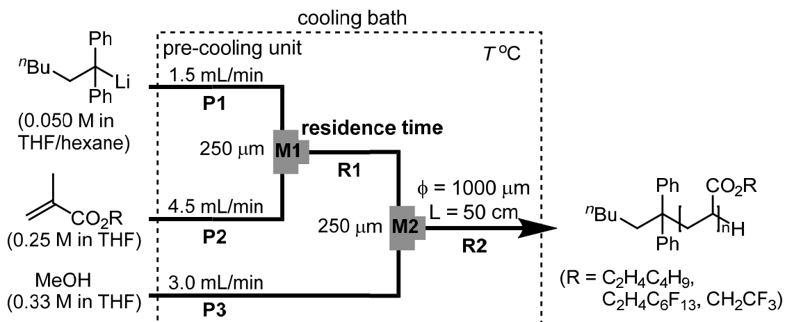
Scheme 1. A flow microreactor system for anionic polymerization of perfluoroalkyl methacrylates initiated by 1,1-diphenylhexyllithium. T-shaped micromixer: M1 , and M2 . Microtube reactor: R1 , and R2 .
