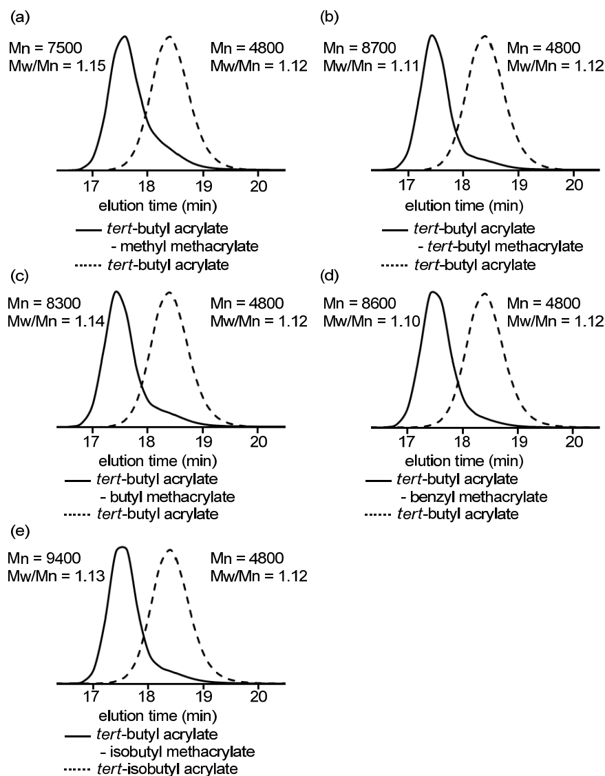
Figure 4. Size exclusion chromatography traces of block copolymers obtained in the integrated flow microreactor system. (a) tert -butyl acrylate (-20 °C)/methyl methacrylate (-20 °C), (b) tert -butyl acrylate (-20 °C)/ tert -butyl methacrylate (20 °C), (c) tert -butyl acrylate (-20 °C)/butyl methacrylate (-20 °C), (d) tert -butyl acrylate (-20 °C)/benzyl methacrylate (-20 °C), (e) tert -butyl acrylate (-20 °C)/isobutyl methacrylate (-20 °C).
