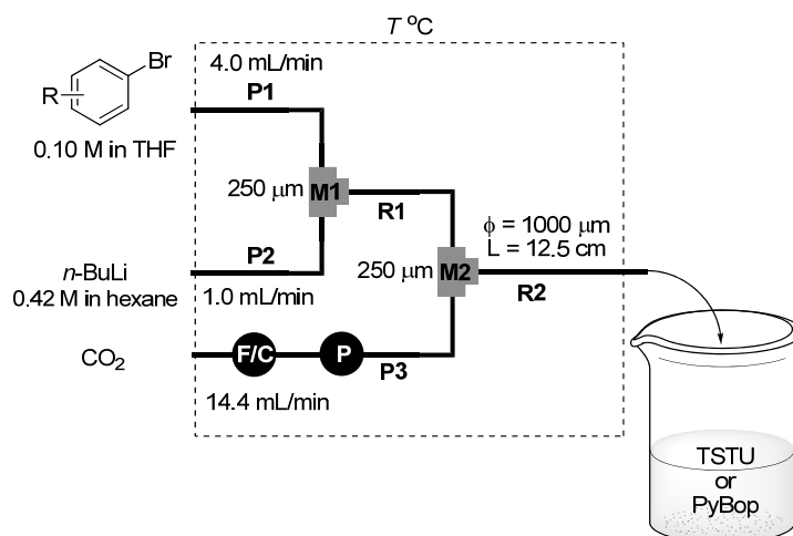
Scheme 3. A flow microreactor system for the synthesis of active esters with \text{CO}_2 gas. T-shaped micromixers: M1 , M2 ; microtube reactors: R1 , R2 ; flow controller: FC; pressure gage: P.
