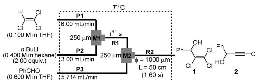
Scheme 1. A flow microreactor system for the H/Li exchange of trichloroethene with n -BuLi (2.00 eq) and the subsequent reaction with electrophiles. T-shaped micromixers: M1 and M2 , microtube reactors: R1 and R2 .
