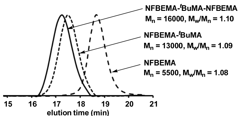
Figure 4. Size exclusion chromatography traces of block copolymers obtained in the integrated flow microreactor system.
