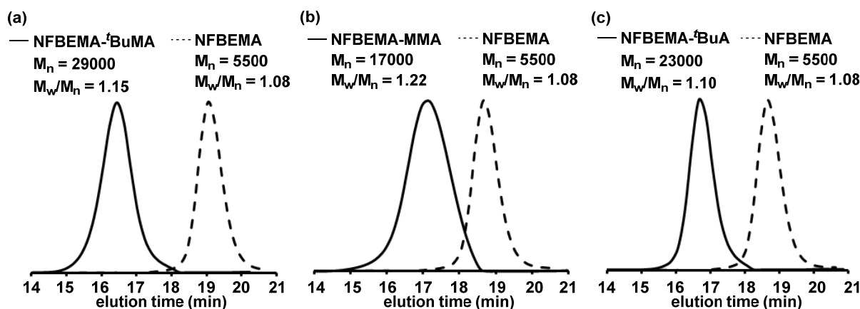
Figure 3. Size exclusion chromatography traces of block copolymers obtained in the integrated flow microreactor system. (a) 2-(Nonafluorobutyl) ethyl methacrylate (NFBEMA) ( -40\text{ }^{\circ}\text{C} )– tert -butyl methacrylate ( t BuMA) ( 20\text{ }^{\circ}\text{C} ), (b) 2-(nonafluorobutyl)ethyl methacrylate (NFBEMA) ( -40\text{ }^{\circ}\text{C} ) – methyl methacrylate (MMA) ( -30\text{ }^{\circ}\text{C} ), and (c) 2-(nonafluorobutyl)ethyl methacrylate (NFBEMA) ( -40\text{ }^{\circ}\text{C} ) – tert -butyl acrylate ( t BuA) ( -20\text{ }^{\circ}\text{C} )
