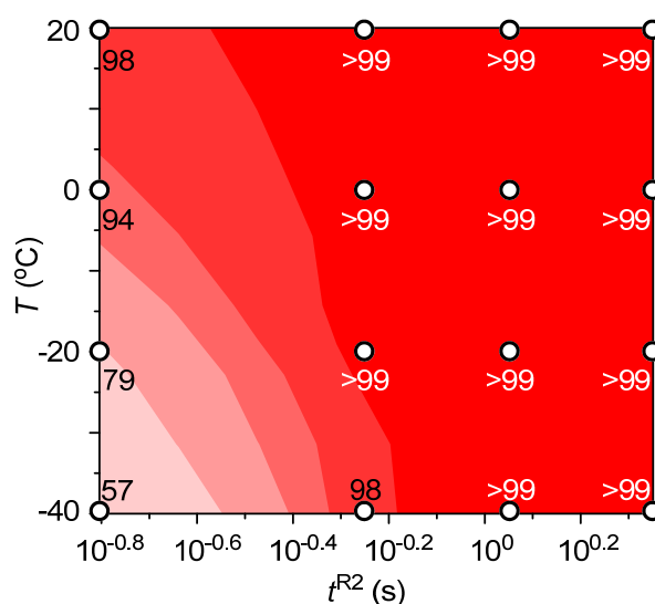
Figure 1. Temperature/residence time map. Contour plots with scatter overlay of the conversion of tert -butyl acrylate, which are indicated by numbered circles.
