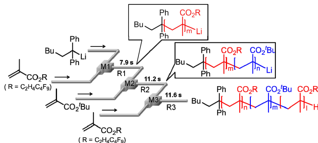
Figure 7. Controlled anionic polymerization of perfluoroalkyl methacrylates to obtain block copolymers.
