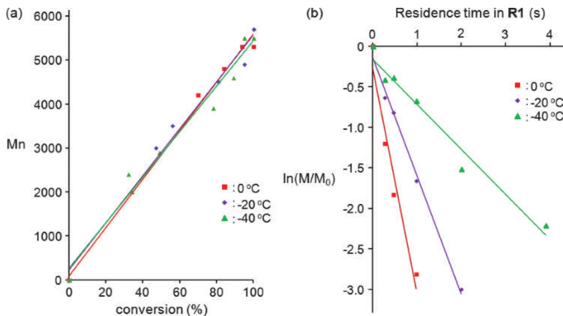
Figure 1. Anionic polymerization of 2-(nonafluorobutyl)ethyl methacrylate initiated by 1,1-diphenylhexyllithium. (a) Plots of M_n against the conversion and (b) plots of \ln(M/M_0) against the residence time in R1
