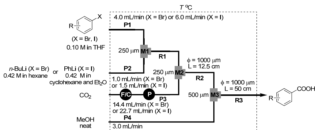
Scheme 1. A flow microreactor system for the reactions of aryllithiums with CO 2 gas. T-shaped micromixers: M1 , M2 , M3 ; microtube reactors: R1 , R2 , R3 ; flow controller: FC; pressure gage: P.
