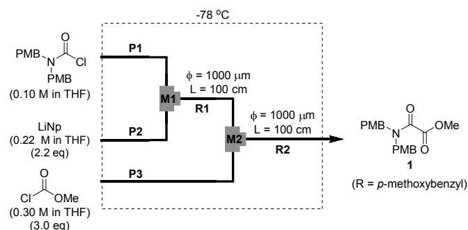
Figure 1. A flow microreactor system for generation of the carbamoyllithium followed by the reaction with methyl chloroformate
