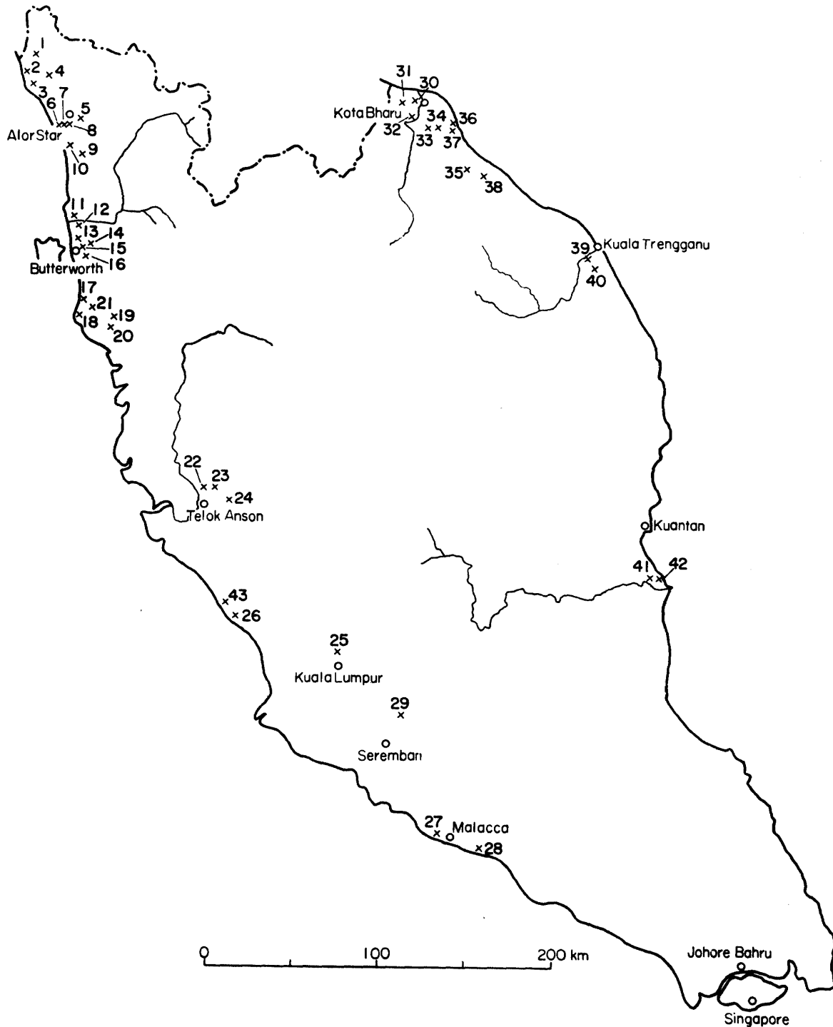
Fig. 11 Map showing Sampling Sites in West Malaysia
