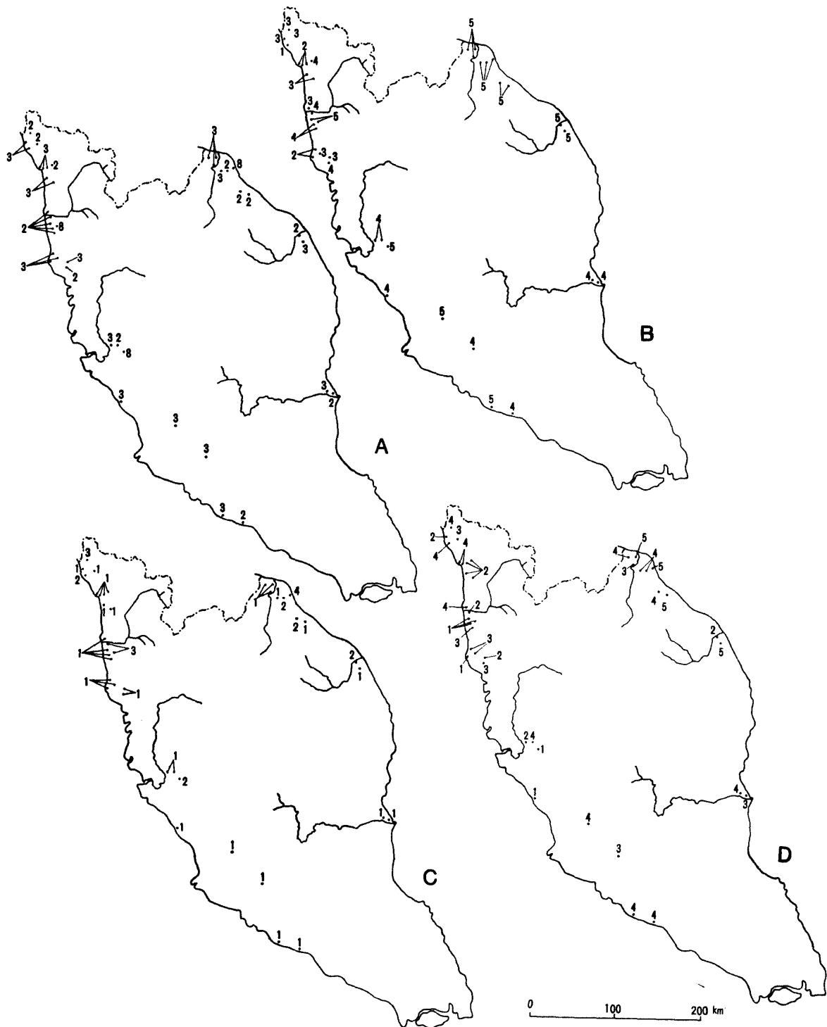
Fig. 12 Map of W. Malaysia, showing Distribution of Samples in Terms of Soil Material and Fertility Characteristics.
