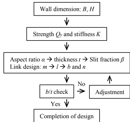
Fig. 12. Flow chart of design procedure
