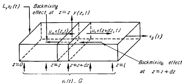
Fig. 4. Material balance on a plate for "diffusional model"
