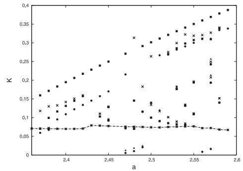
Fig. 9. The second-largest Lyapunov exponent changes from positive to zero (●), from zero to negative (■), from negative to zero (×), and from zero to positive (▲), as the coupling strength K is increased for the bidirectional coupling. The CPS transition points given by Eq. (1.6) are plotted with the symbol (*) together with a solid line in the a - K plane.
