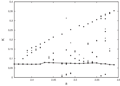
Fig. 8. The symbols (●) and (▲) are plotted on the K - a plane where the largest Lyapunov exponent changes from positive to a constant value of zero and from a constant value of zero to positive, respectively, as the coupling strength K is increased for the bidirectional coupling. The CPS transition points given by Eq. (1.6) are plotted with the symbol (*) together with a solid line in the a - K plane.
