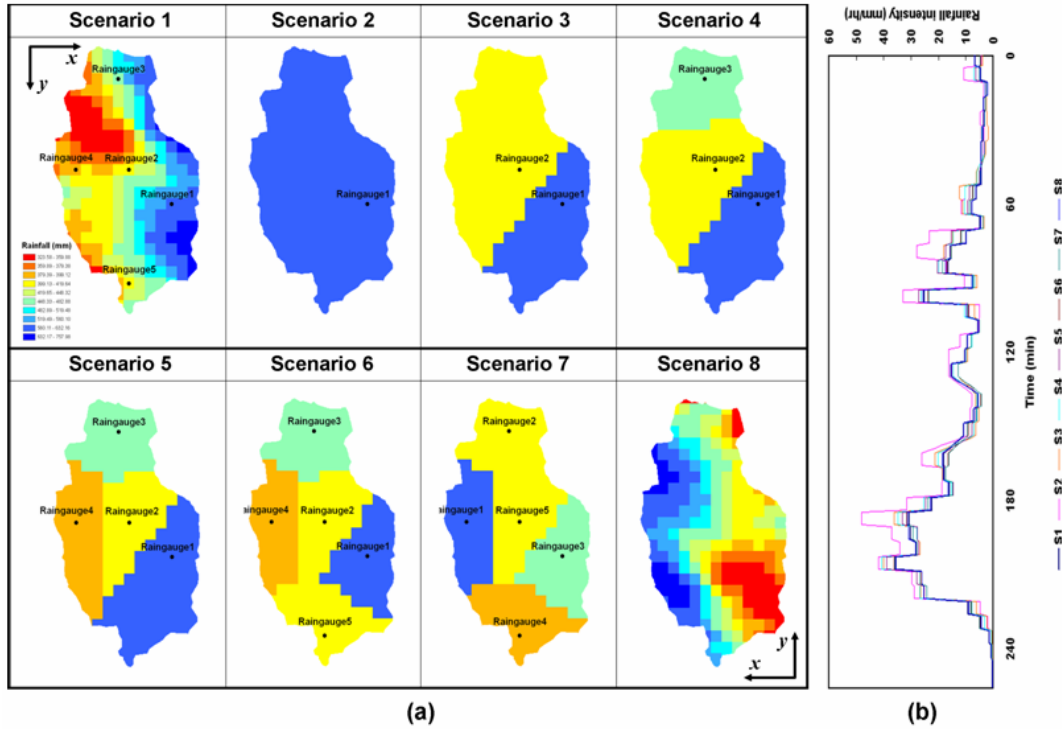
Fig. 6 (a) Spatial patterns of accumulated rainfall and (b) time series of areal mean rainfall for all rainfall scenarios of Event1.
