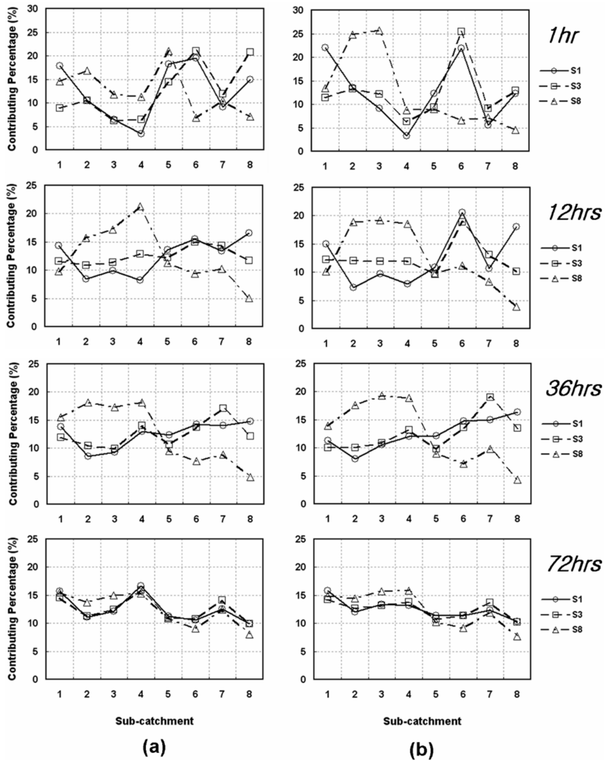
Fig. 12 Variation of the Contributing Percentage (CP) of each sub-catchment due to mimic rainfall scenarios for Event 1; (a) 250m-based and (b) 500m-based results.
