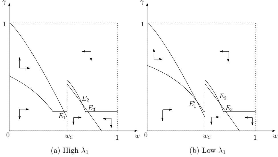
Figure 4: Bubbly traps
