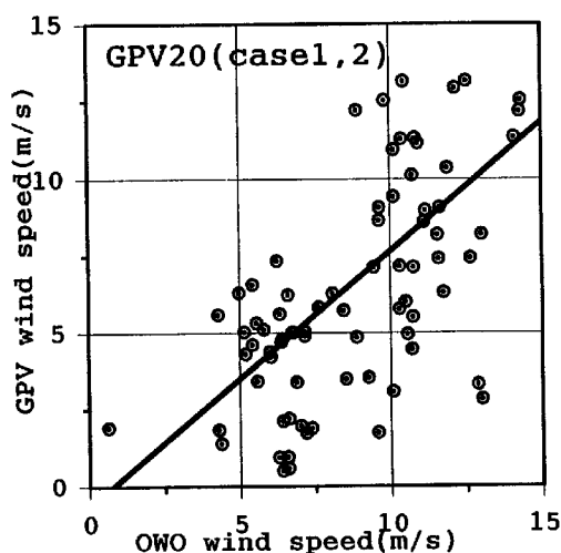
Fig.14 GPV's surface wind vs observed wind at the pier of Ogata Wave Observatory.
