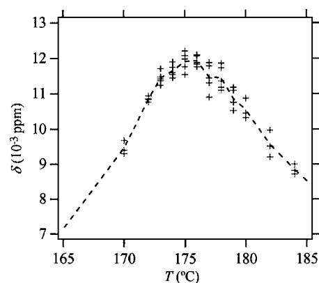
FIG. 1. The chemical shift \delta plotted against temperature for the sample at the lowest density of 0.0046\text{ g cm}^{-3} . The \delta for the gas branch of the liquid-gas coexistence curve at 150\text{ °C} ( 0.0025\text{ g cm}^{-3} ) is set to zero. The dashed line indicates the average of the repetitions.
