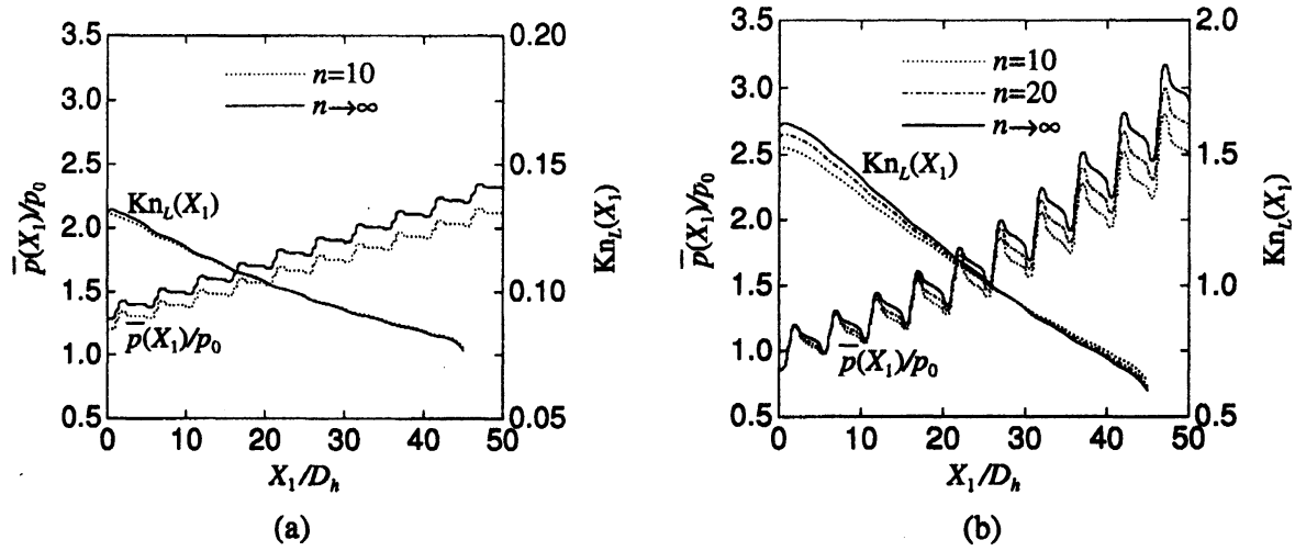
Fig. 9: The distribution of the average pressure \bar{p}(X_1) and local Knudsen number Kn_L(X_1) in the steady state of a closed system of 10 compressor units (Problem II). T_h/T_c = 3 . .....: n = 10 , — · —: n = 20 , —: n \rightarrow \infty . (a) Kn=0.1 , (b) Kn=1 .
