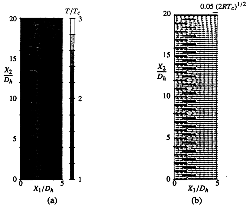
Fig. 5: One way flow in the thermal edge compressor II ( Problem I ). T_h/T_c = 3 , n = 40 , and \text{Kn} = 1 . (a) Temperature field and (b): flow velocity field. (See the caption of Fig. 4).
