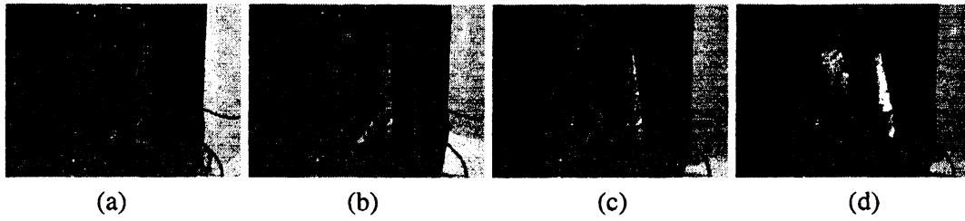
Fig. 15: The movement of the film in experiment (A) for the case of channel width of 1mm. I: The results for constant pressure p=1\text{Pa} and various energy supply E to the heater. (a) E = 0\text{W} , (b) 5.2\text{W} , (c) 12\text{W} , and (d) 21\text{W} .
