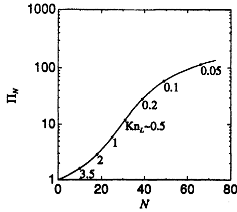
Fig. 11: The compression ratio \Pi_N obtained by N compressor units ( Problem II ). T_h/T_c = 3, n \rightarrow \infty, \text{Kn}_{L(1)} = 5.7 . The marks \bullet show the points (i, \Pi_i) where \text{Kn}_{L(i)} \sim 0.05, 0.1, 0.2, 0.5, 1, 2, 3.5 .
