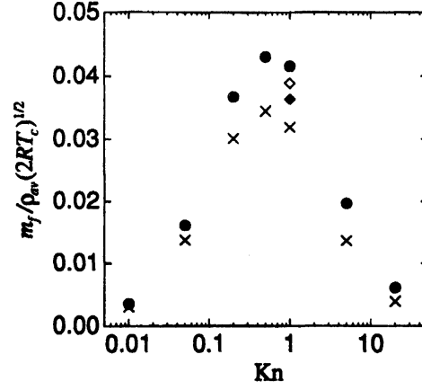
Fig. 7: Nondimensional mass flow rate per cross sectional area m_f / \rho_{av} (2RT_c)^{1/2} vs Knudsen number Kn of the thermal edge pump ( Problem-I ). T_h/T_c = 3 . \times : n = 10 , \diamond : n = 20 , \diamond : n = 40 , \bullet : n \rightarrow \infty .
