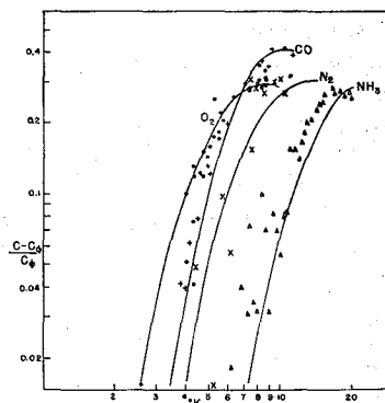
Fig. 4. Relative heat capacity of oxygen, \circ ; carbon monoxide, + ; nitrogen, \times ; and ammonia, \triangle ; compared to theory in high temperature form. Curves must necessarily converge upon low temperature approximation.
