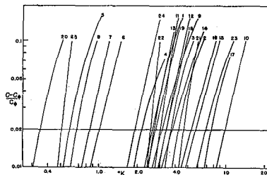
Fig. 2. Relative heat capacity as a function of temperature in the low temperature approximation for substances of Table II. Symbols from Table II.
