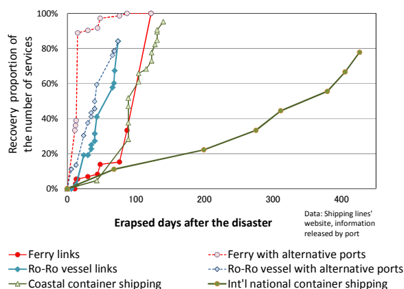
Fig. 10 Resiliency of liner shipping (Performance observed at the East Japan Great Earthquake) (see Ono, 2012)
