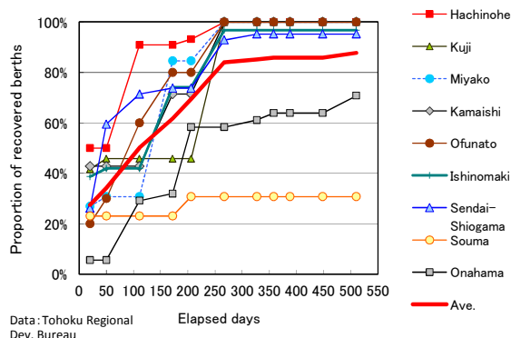
Fig. 4 Rehabilitation of damaged public wharves (ratio of the rehabilitated berths) (see Ono et al, 2013)
