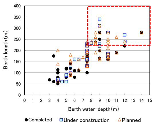
Fig. 11 Berth specifications of high earthquake resistance berths in Japan (Ono (2013b))
