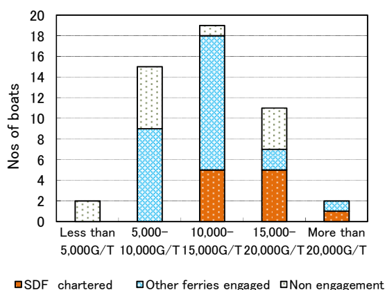
Fig. 9 Ship size of the long distance ferryboats mobilized for ERL operation at the East Japan Great Earthquake
