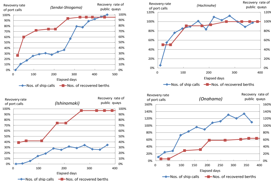
Fig. 6 Recovery rates of commercial ship calls and public quays at the disaster ports (see Ono et al, 2013a)
