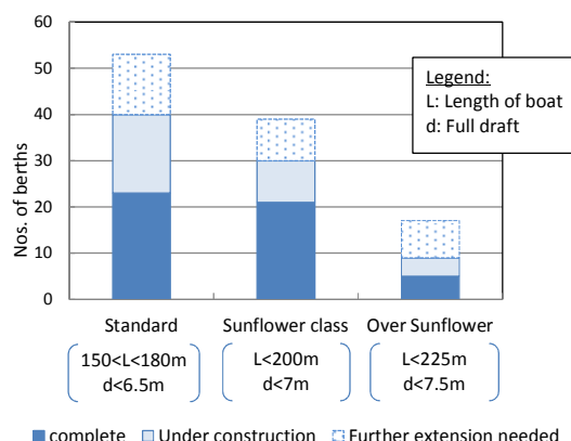
Fig. 12 High earthquake resistance berths for accommodating mega-ferries (Ono (2013b))
