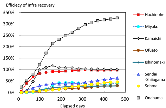
Fig. 8 Efficiency indices of rehabilitated public berth in major Tohoku ports (Ono, et al (2013))
