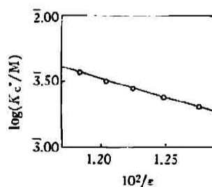
Fig. 6 \log K_e^* vs. reciprocal dielectric constant at 25°C
