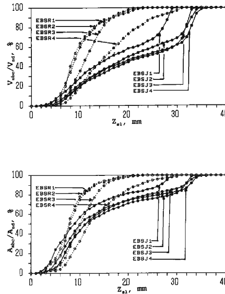
Fig. 5. Relations between V_{sbc}/V_{sd} , A_{sbc}/A_{sd} and Z_{sl} .
