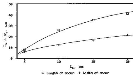
Fig. 6. Relation between L_s , W_s and L_b in the experiments EBSR.
