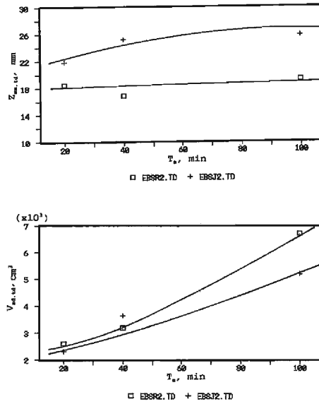
Fig. 16. Relations between Z_{\max,td} , V_{ad,td} and T_e .
