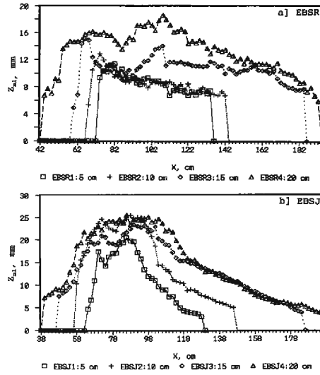
Fig. 8. Z_m along x in the experiments EBSR and EBSJ.
