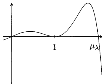
Figure 2: The graph of H_\lambda for \lambda > -\frac{1}{2} .
