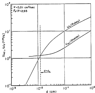
Fig. 1. The critical states of particles in flowing water.
