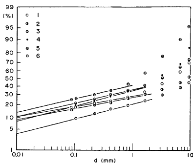
Fig. 4. Grain size accumulation curves of materials sampled in the Naka River basin.
