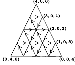
FIGURE 1. A subdivision into n^2 triangles ( n = 4 ).
