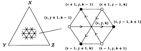
FIGURE 2. The black (resp. white) vertices correspond to the factors of the numerator (resp. denominator) of the triple ratio.
