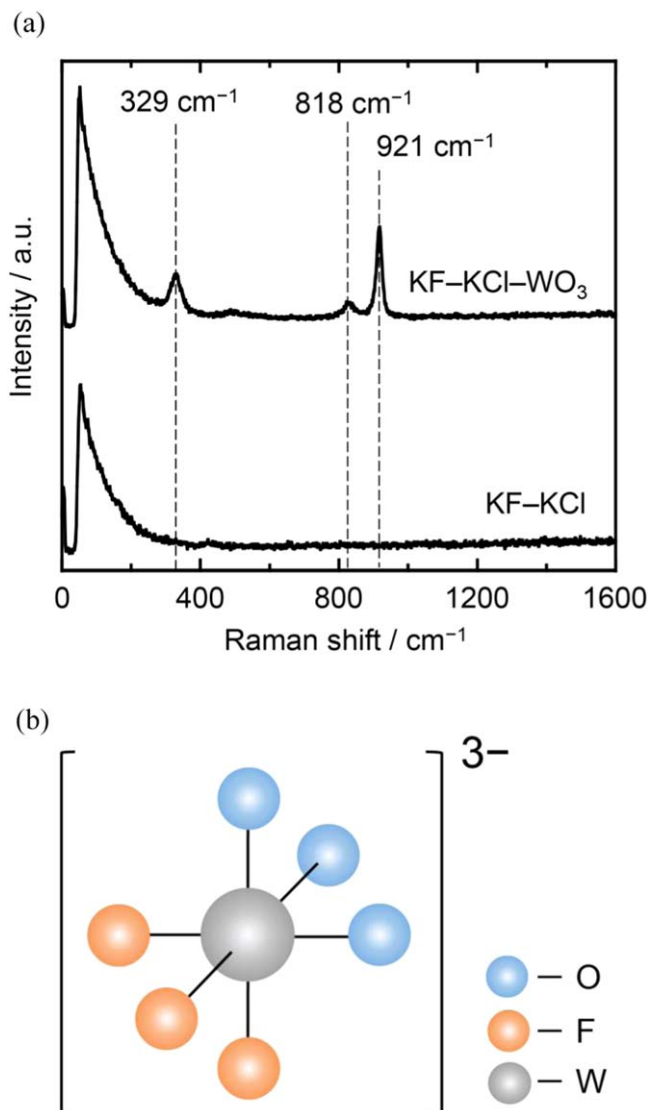
Figure 1. (a) Raman spectra of molten KF-KCl and molten KF-KCl-WO 3 (2.0 mol% added) at 923 K. (b) Structure of fac -[WO 3 F 3 ] 3- ion.
