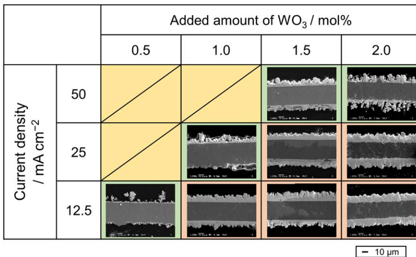
Figure 7. Cross-sectional SEM images of the samples obtained by galvanostatic electrolysis of Cu foil electrodes at various current densities and added amounts of \text{WO}_3 in molten \text{KF-KCl} at 923 K. Charge density: 90 \text{ C cm}^{-2} . The scale bar is common for all images.
