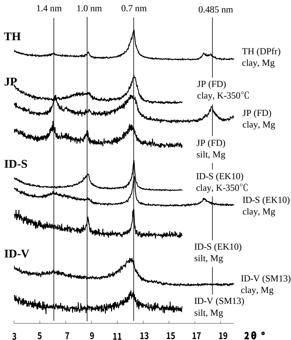
Fig. 2.2. X-ray (Cu-Kα) diffractograms from oriented specimens from silt and clay fractions.
