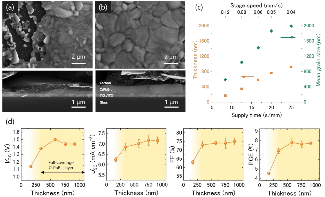
Figure 3. (a, b) Surface and cross-sectional SEM images of CsPbBr 3 PSCs with CsPbBr 3 layer deposited at stage speeds of (a) 0.12, and (b) 0.06 \text{mm s}^{-1} , respectively. (c) Correlation between supply time, film thickness, and mean grain size. (d) Photovoltaic performance, including J_{sc} , V_{oc} , FF, and PCE, of the CsPbBr 3 PSCs with CsPbBr 3 layers of various thicknesses.
