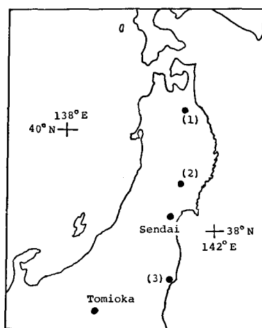
Fig. 18. Map showing the locations of the Kadosawa-Sannohe (1), Ichinoseki (2), and Joban (3) areas, northern Japan.
