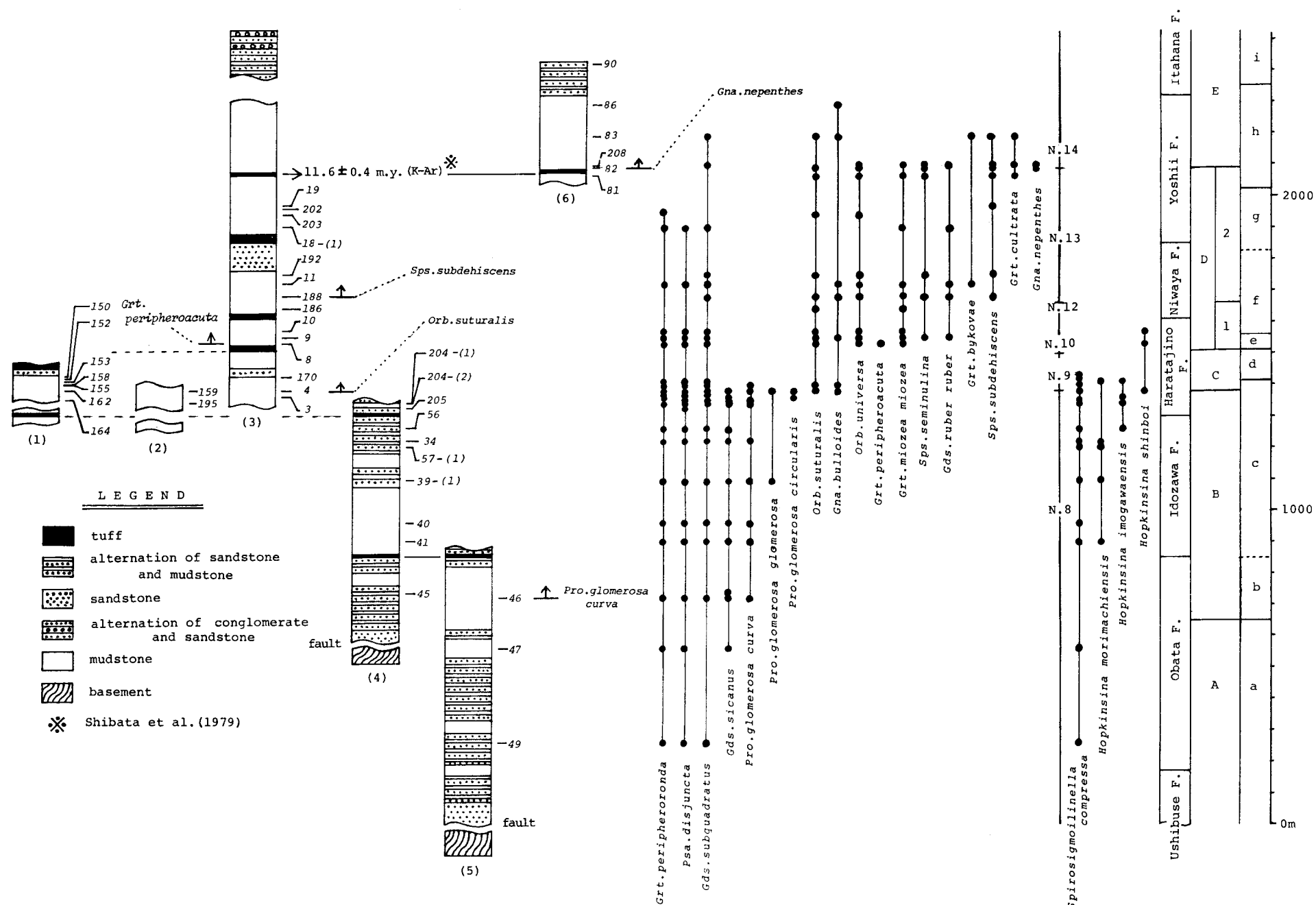
Fig. 3. Columnar sections of the Tomioka Group showing stratigraphic positions of samples and stratigraphic distribution of some selected planktonic and benthonic foraminifera.
