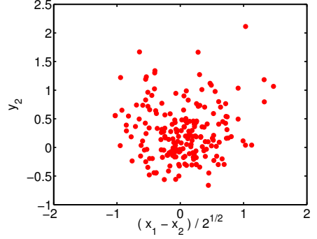
Figure 3: Relationship between (x_1 - x_2) / \sqrt{2} and y_2 in dataset (c). There seems no strong dependency between these two quantities.
