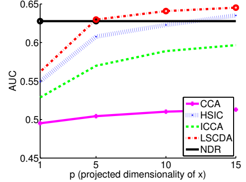
Figure 4: Comparison of the average AUC score for the PASCAL VOC 2010 dataset. The best method and comparable methods according to the t -test at the significance level 1% are specified by “o”. “NDR” denotes the original data without dimension reduction. The horizontal axis is corresponding to projected dimensionality of \mathbf{x} (i.e., dimensionality of \mathbf{u} ).
