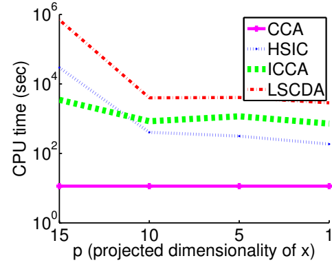
Figure 7: CPU time comparison of dimensionality reduction. The horizontal axis is corresponding to projected dimensionality of \mathbf{x} (i.e., dimensionality of \mathbf{u} ).
