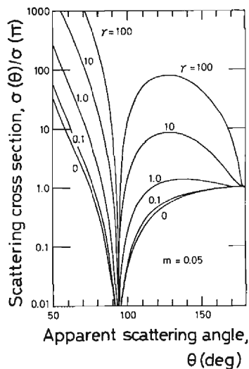
Fig. 2 Scattering cross section as a function of apparent scattering angle with ratio m of mean wind to speed of sound and r = C_v^2 T^2 / C_T^2 C^2 as parameters (after Brown, E.H. 32) )
