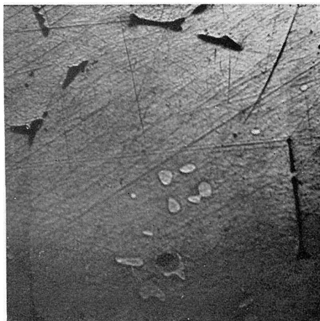
Fig. 8. ×150 24 wt. % Au, air-cooled and annealed for 60 hours at 200^\circ\text{C} ( \text{AuPb}_3 + \text{AuPb}_2 +eutectic)
