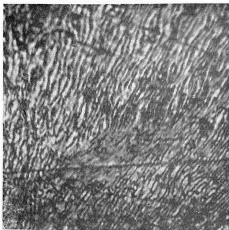
Fig. 2. \times 800 15 wt. % Au, air-cooled (eutectic)
