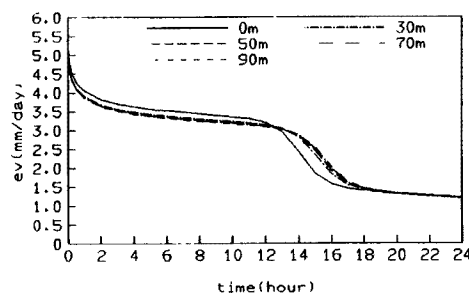
Fig. 6. Changes of the evaporation rate with time. (Case. 1)
