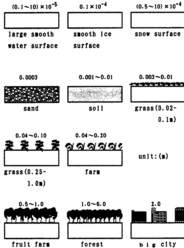
Fig. 5. Roughness length values for various land surfaces.
