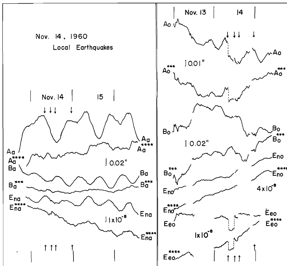
Fig. 13. Tilting motions and variations of linear strain before and after the remarkable local earthquakes on Nov. 14, 1960. (×××× : corrected curve, ↑ : local earthquake)
