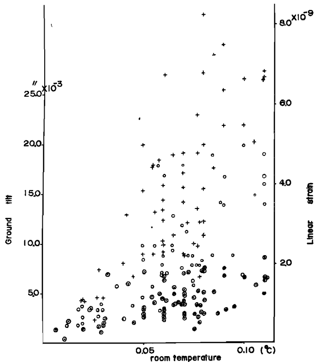
Fig. 11. Relation between the ground the tilt, linear strain and the room temperature.
