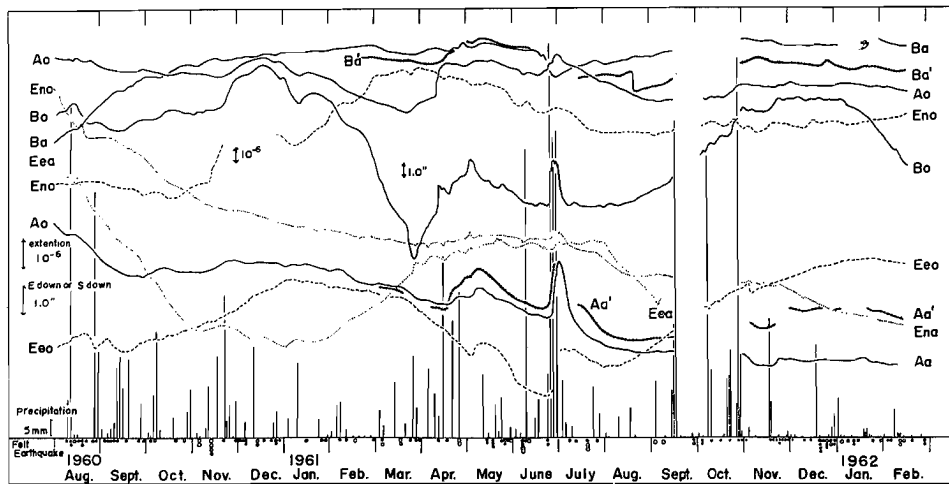
Fig. 6. Tilting motion and variation of linear strain observed at Oura and Akibasan. (○ : Remarkable local earthquakes, ● : Felt local earthquakes, Vertical line : precipitation)
