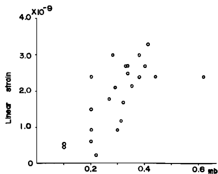
Fig. 9d. Relation between the linear strain and the pressure change.
