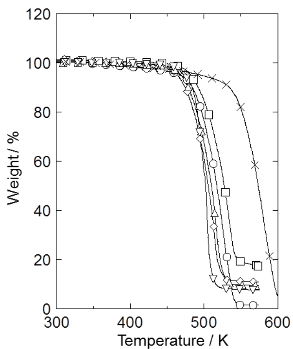
Fig. 2 Thermogravimetric curves of C_3MIm(FH)_{1.7}F (×), C_{3F_3}MIm(FH)_{1.7}F (○), C_{4F_5}MIm(FH)_{1.7}F (□), C_{6F_9}MIm(FH)_{1.8}F (◇), C_{8F_{13}}MIm(FH)_{2.0}F (△), and C_{10F_{17}}MIm(FH)_{2.0}F (▽).
