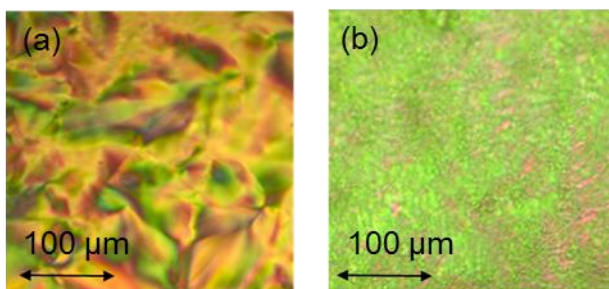
Fig. 6 Polarized optical microscopic textures of (a) C_{8F_{13}}MIm(FH)_{2.0}F at 373 K on cooling from isotropic liquid phase and C_{10F_{17}}MIm(FH)_{2.0}F at 373 K on heating from crystal phase.
