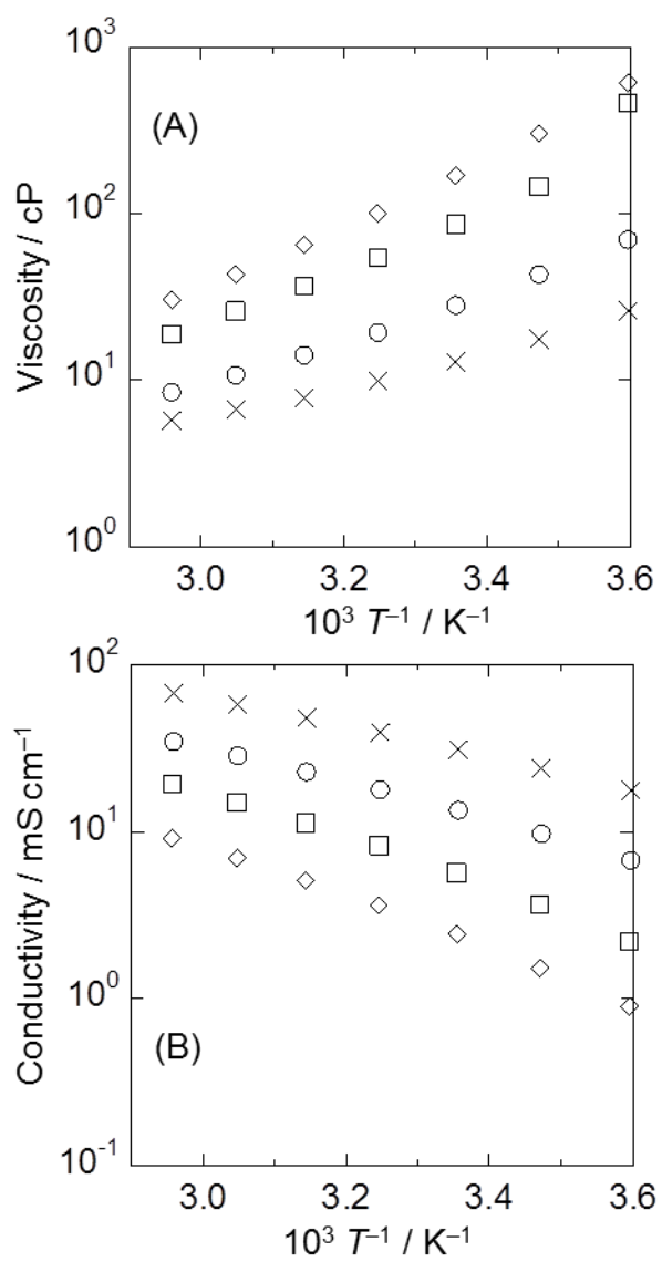
Fig. 4 Arrhenius plots of (A) viscosity and (B) ionic conductivity for \text{C}_3\text{MIm}(\text{FH})_{1.7}\text{F} (x), \text{C}_{3\text{F}_3}\text{MIm}(\text{FH})_{1.7}\text{F} (o), \text{C}_{4\text{F}_5}\text{MIm}(\text{FH})_{1.7}\text{F} (□), and \text{C}_{6\text{F}_9}\text{MIm}(\text{FH})_{1.8}\text{F} (◇).
