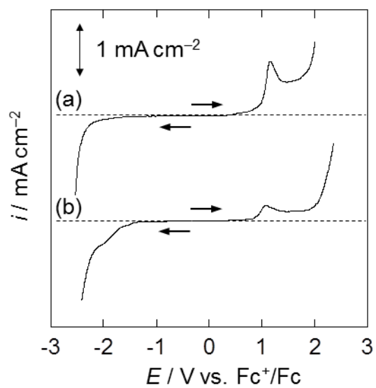
Fig. 5 Linear sweep voltammograms of a vitreous carbon electrode in (a) \text{C}_3\text{MIm}(\text{FH})_{1.7}\text{F} , (b) \text{C}_{3\text{F}_3}\text{MIm}(\text{FH})_{1.7}\text{F} . Scan rate: 10 \text{ mV s}^{-1} .
