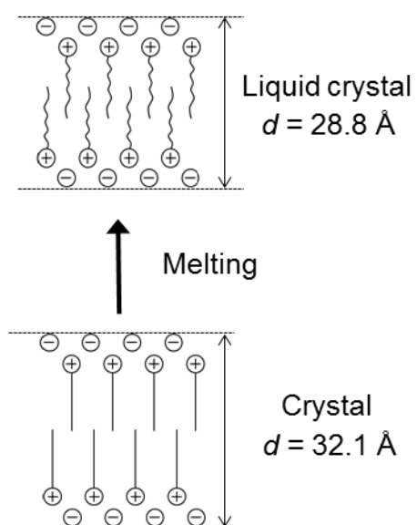
Fig. 9 Schematic illustration of the crystal–liquid crystal phase transition of \text{C}_{8\text{F}_{13}}\text{MIm}(\text{FH})_{2.0}\text{F} .
