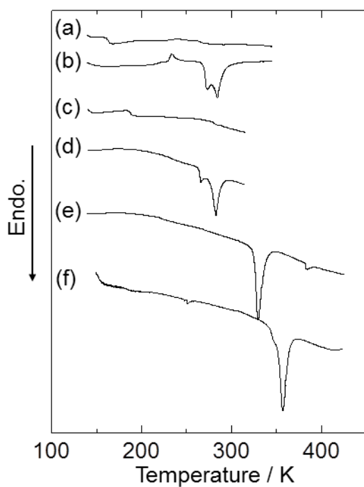
Fig. 3 Differential scanning calorimetric curves of (a) C_3\text{MIm}(\text{FH})_{1.7}\text{F} , (b) C_{3\text{F}_3}\text{MIm}(\text{FH})_{1.7}\text{F} , (c) C_{4\text{F}_5}\text{MIm}(\text{FH})_{1.7}\text{F} , (d) C_{6\text{F}_9}\text{MIm}(\text{FH})_{1.8}\text{F} , (e) C_{8\text{F}_{13}}\text{MIm}(\text{FH})_{2.0}\text{F} , and (f) C_{10\text{F}_{17}}\text{MIm}(\text{FH})_{2.0}\text{F} .
