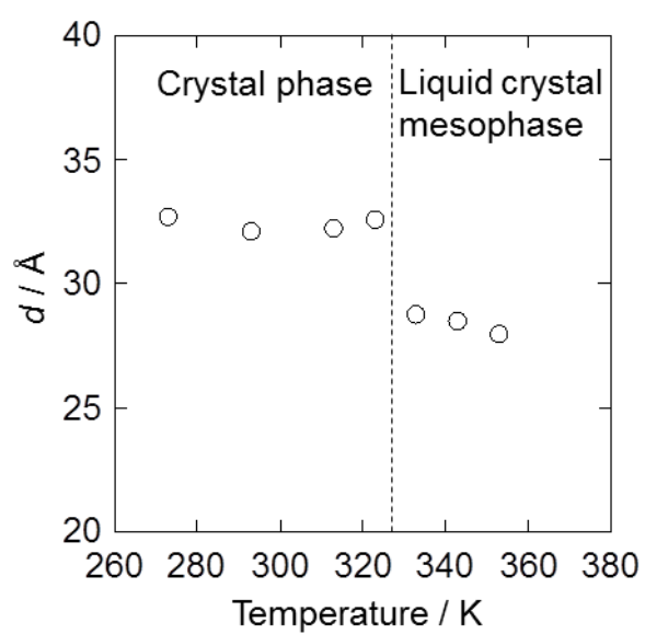
Fig. 8 Layer spacing of C_{8F_{13}}MIm(FH)_{2.0}F in the crystal phase and liquid crystal phase at different temperatures.
