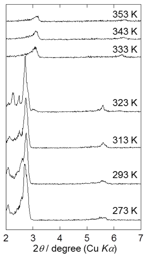
Fig. 7 X-ray diffraction patterns in the low-angle region for C_{8F_{13}}MIm(FH)_{2.0}F in the crystal phase (273–323 K) and the liquid crystal phase (333–353 K).
