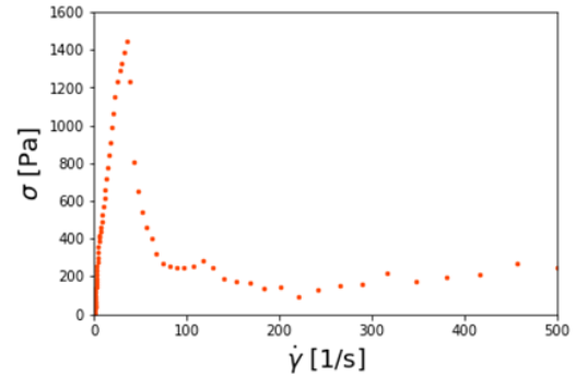
Fig. 2 Stress measurement under the steady shear rate.
