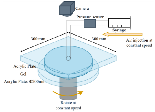
Fig. 3 Experimental setup.
