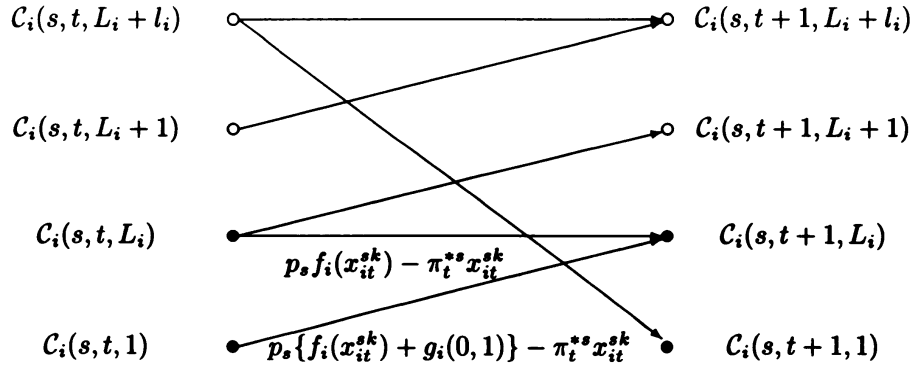
Figure 3: Recursive equation of dynamic programming( L_i = l_i = 2 )
