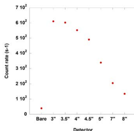
Fig. 1. Results of Bonner sphere measurements.
