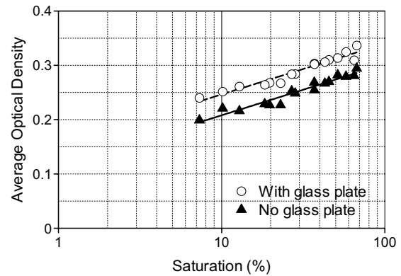
Fig. 3 Effect of the glass plate on the D_i - S curve
