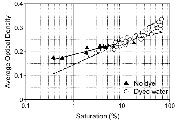
Fig. 2 Effect of blue dye on the slope of D_i - S curve
