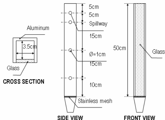
Fig. 4 Column design
