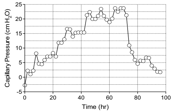
Fig. 13 Capillary pressure vs. time ( h = 25 cm)
