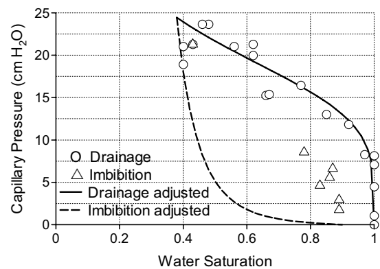
Fig. 14 S - p relation
