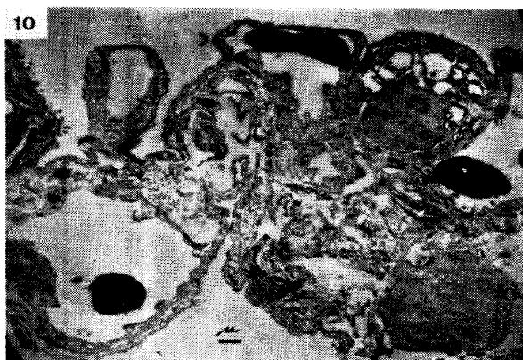
Fig. 10. Alveolar wall-cell, lung, rabbit ( \times 6000 )
