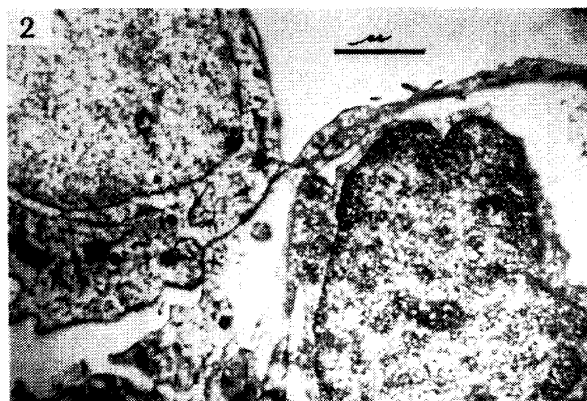
Fig. 2. Nucleated alveolar epithelium, lung, guinea-pig ( \times 24000 )
