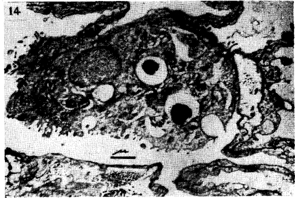
Fig. 14. Alveolar wall-cell, lung, guinea-pig ( \times 13700 )
