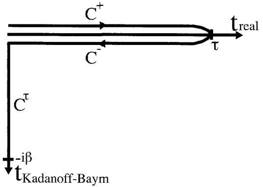
図9 Kadanoff-Baym 経路
