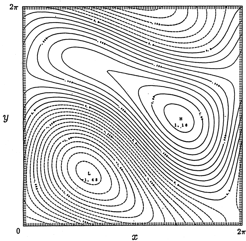
Figure 3. Initial contours of the vorticity field \omega(x, 0) . Positive or negative extremum is denoted by the symbol H or L, respectively.
