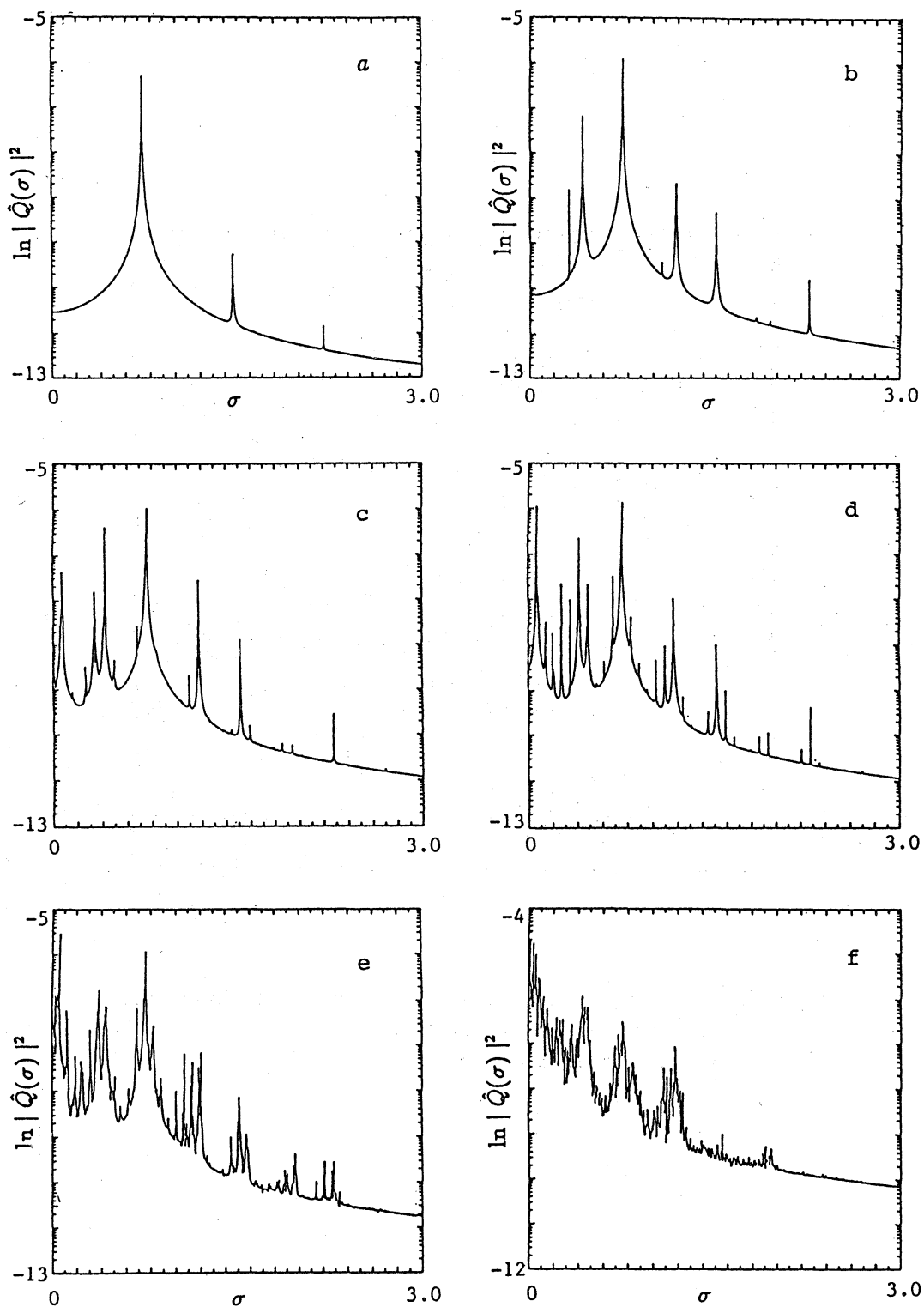
Figure 5. Frequency power spectrum \ln |\dot{Q}(\sigma)|^2 for the cases corresponding to Figure 4.
