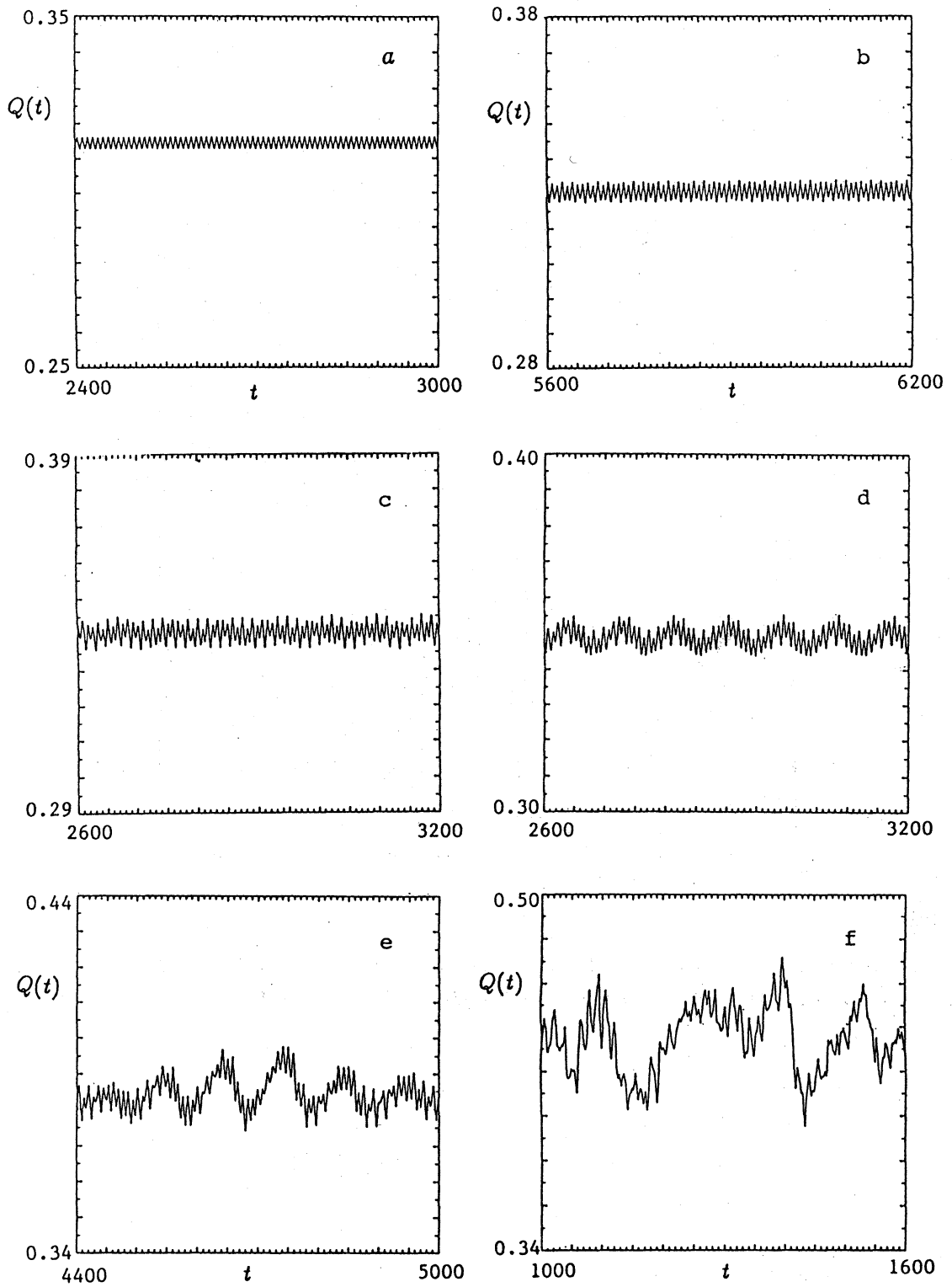
Figure 4. Temporal behaviors of the enstrophy Q(t) for the viscosity \nu : (a) 0.0020, (b) 0.00156, (c) 0.0014, (d) 0.0013, (e) 0.0010 and (f) 0.0006.
