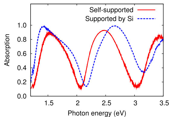
FIG. 3. Optical absorption spectra of self-supported local plasmon resonator (red solid line) and resonator supported by Si wafer (blue dashed line).
