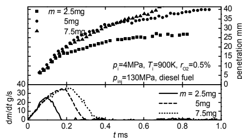
Fig.3 Effect of injection quantity on spray penetration
