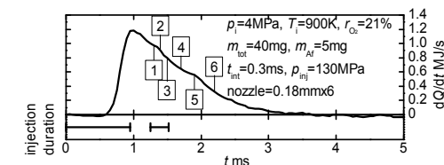
Fig.1 Images of luminous flame and heat release rate
